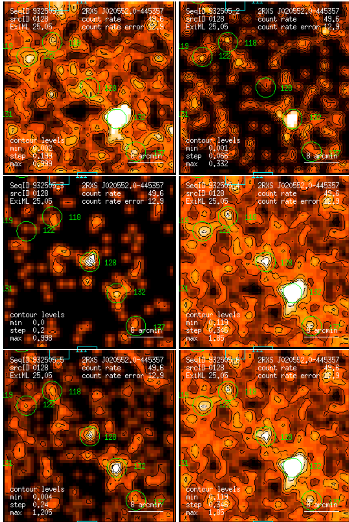
Figure 128: RASS 932505: detection 0128: band rate images, Gaussian filter: (1) PSPC channels 11 – 41, (2) 52 – 90, (3) 91 – 201, (4) 11 – 235, (5) 52 – 201, (6) 11 – 201. Broad band rates in counts/ks. Band rate contour levels in counts/ks/arcmin 2 .
