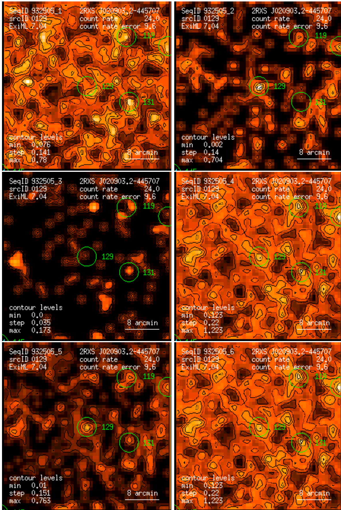
Figure 129: RASS 932505: detection 0129: band rate images, Gaussian filter: (1) PSPC channels 11 – 41, (2) 52 – 90, (3) 91 – 201, (4) 11 – 235, (5) 52 – 201, (6) 11 – 201. Broad band rates in counts/ks. Band rate contour levels in counts/ks/arcmin 2 .
