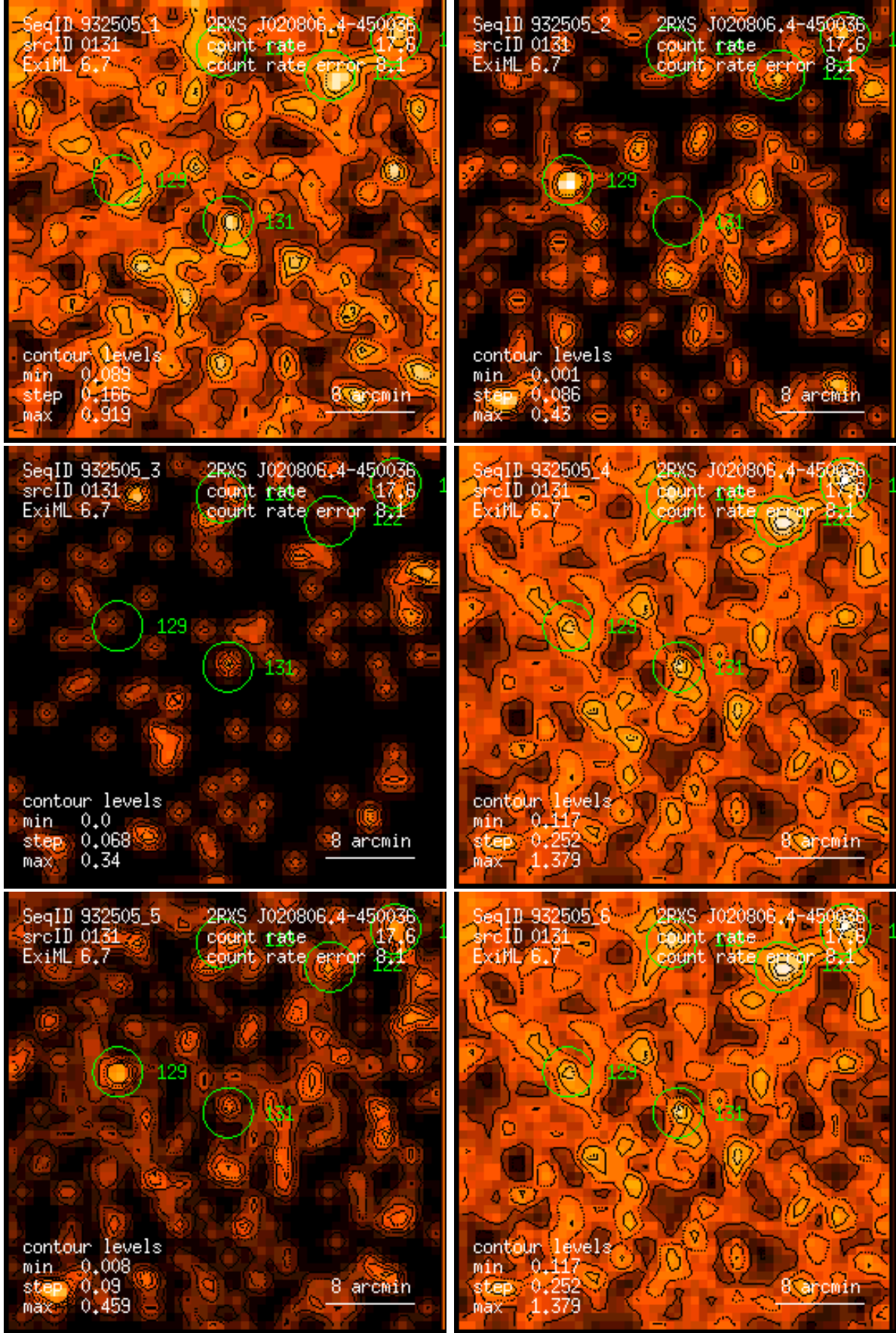
Figure 131: RASS 932505: detection 0131: band rate images, Gaussian filter: (1) PSPC channels 11 – 41, (2) 52 – 90, (3) 91 – 201, (4) 11 – 235, (5) 52 – 201, (6) 11 – 201. Broad band rates in counts/ks. Band rate contour levels in counts/ks/arcmin 2 .
