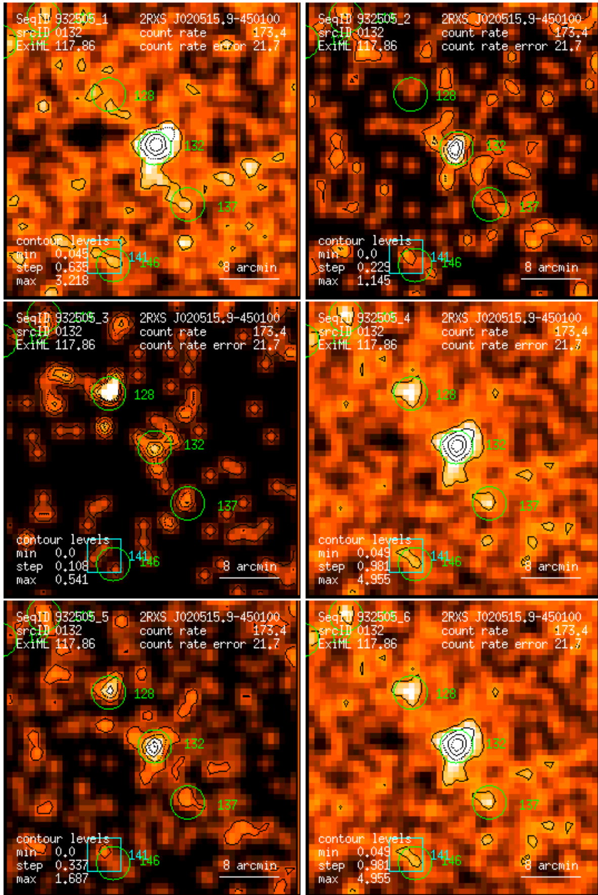
Figure 132: RASS 932505: detection 0132: band rate images, Gaussian filter: (1) PSPC channels 11 – 41, (2) 52 – 90, (3) 91 – 201, (4) 11 – 235, (5) 52 – 201, (6) 11 – 201. Broad band rates in counts/ks. Band rate contour levels in counts/ks/arcmin 2 .
