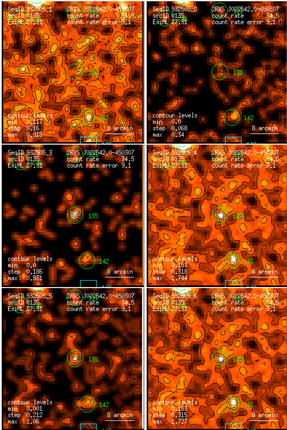
Figure 135: RASS 932505: detection 0135: band rate images, Gaussian filter: (1) PSPC channels 11 – 41, (2) 52 – 90, (3) 91 – 201, (4) 11 – 235, (5) 52 – 201, (6) 11 – 201. Broad band rates in counts/ks. Band rate contour levels in counts/ks/arcmin 2 .
