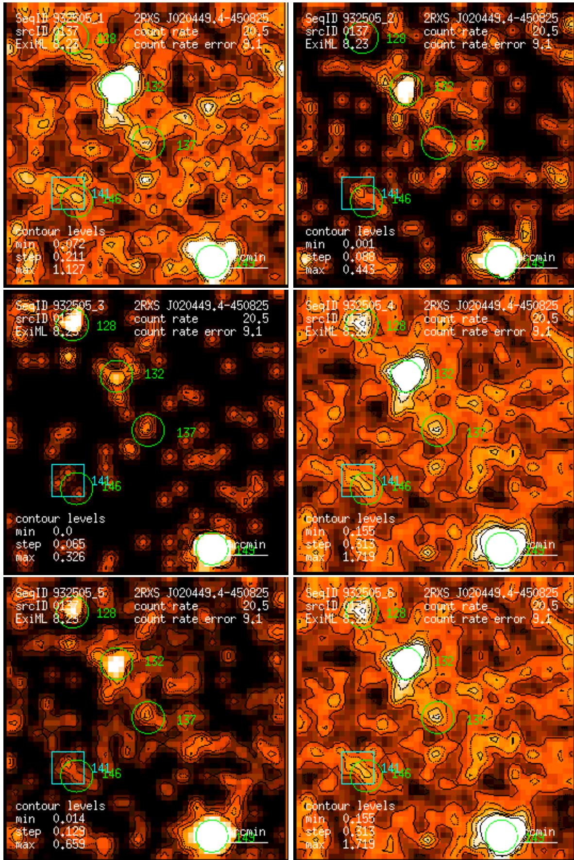
Figure 137: RASS 932505: detection 0137: band rate images, Gaussian filter: (1) PSPC channels 11 – 41, (2) 52 – 90, (3) 91 – 201, (4) 11 – 235, (5) 52 – 201, (6) 11 – 201. Broad band rates in counts/ks. Band rate contour levels in counts/ks/arcmin 2 .
