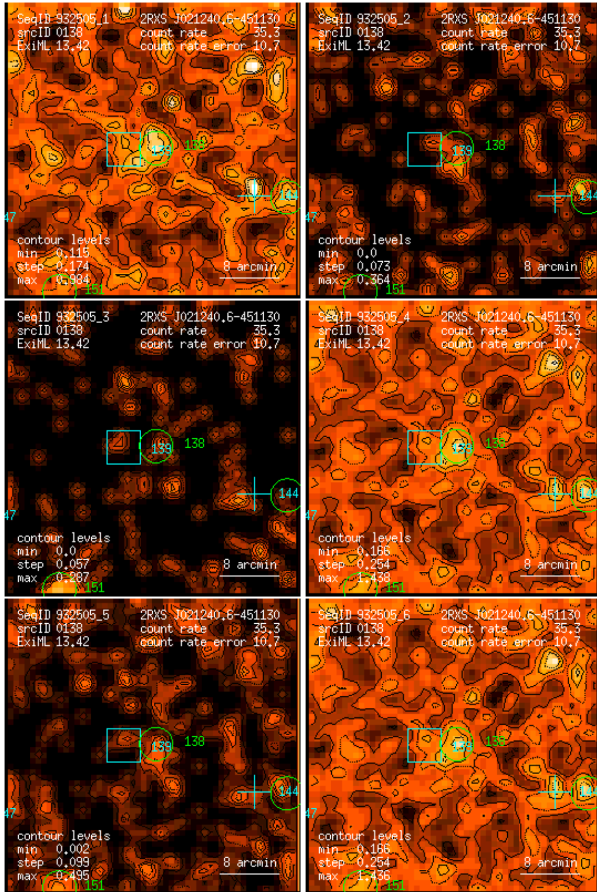
Figure 138: RASS 932505: detection 0138: band rate images, Gaussian filter: (1) PSPC channels 11 – 41, (2) 52 – 90, (3) 91 – 201, (4) 11 – 235, (5) 52 – 201, (6) 11 – 201. Broad band rates in counts/ks. Band rate contour levels in counts/ks/arcmin 2 .
