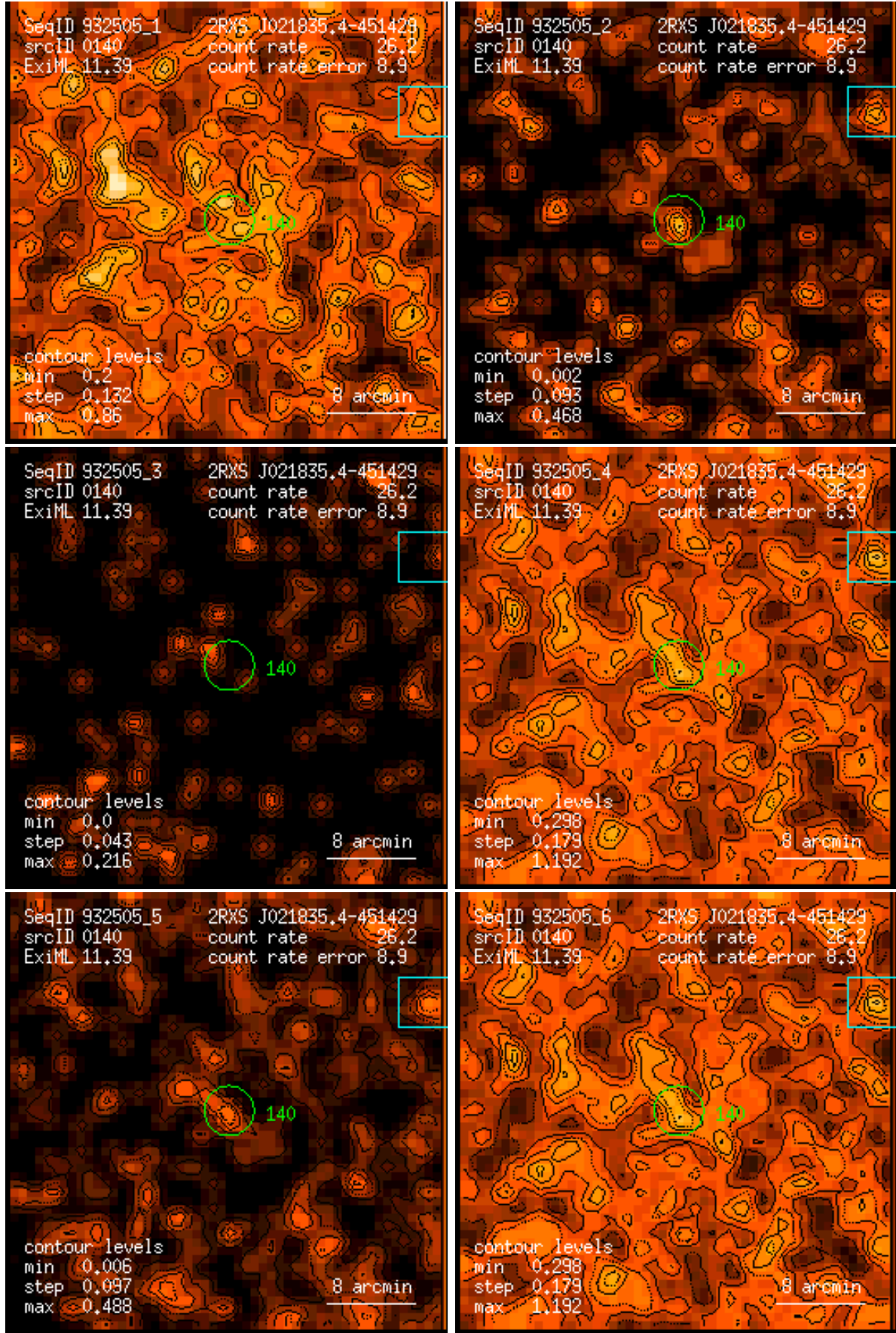
Figure 140: RASS 932505: detection 0140: band rate images, Gaussian filter: (1) PSPC channels 11 – 41, (2) 52 – 90, (3) 91 – 201, (4) 11 – 235, (5) 52 – 201, (6) 11 – 201. Broad band rates in counts/ks. Band rate contour levels in counts/ks/arcmin 2 .
