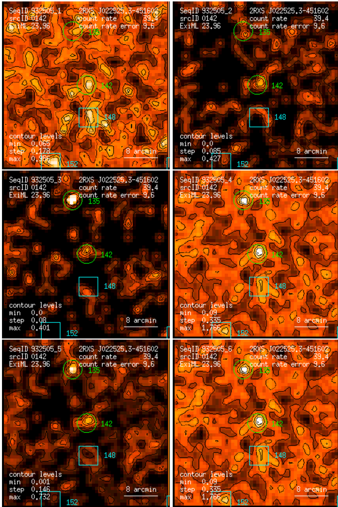
Figure 142: RASS 932505: detection 0142: band rate images, Gaussian filter: (1) PSPC channels 11 – 41, (2) 52 – 90, (3) 91 – 201, (4) 11 – 235, (5) 52 – 201, (6) 11 – 201. Broad band rates in counts/ks. Band rate contour levels in counts/ks/arcmin 2 .
