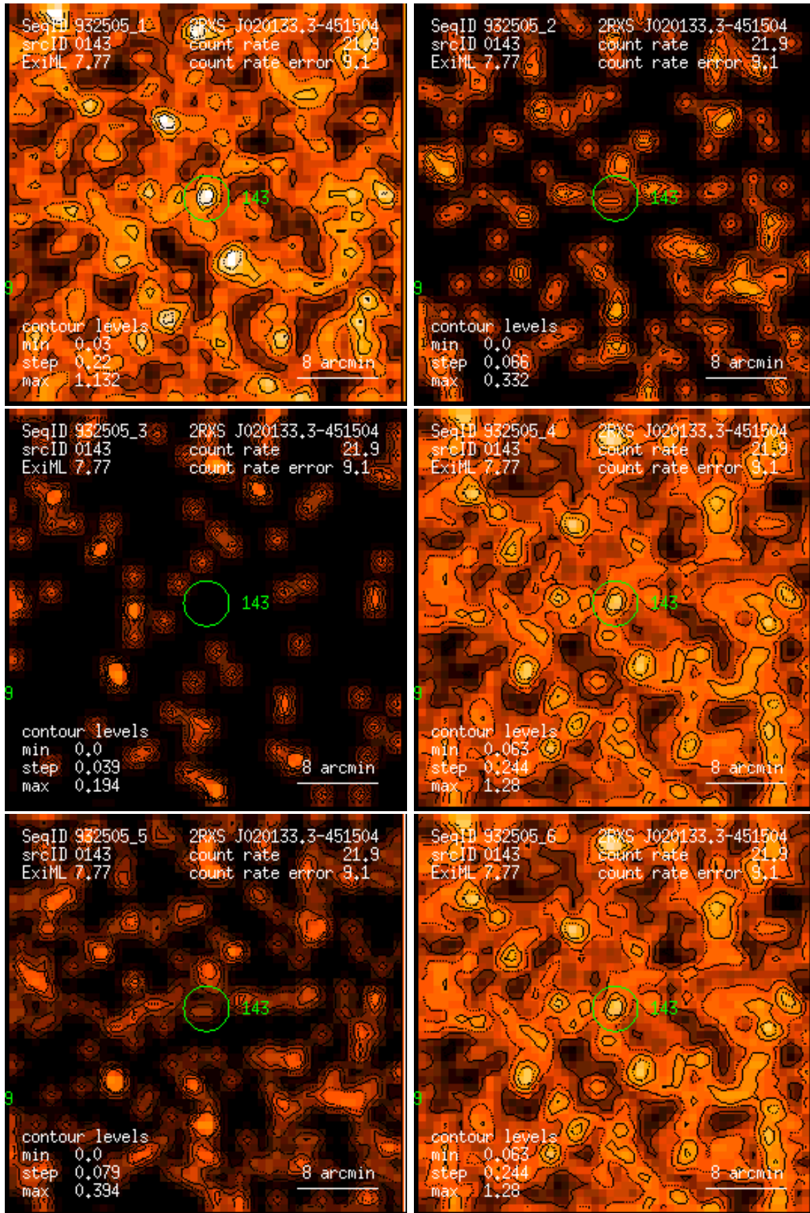
Figure 143: RASS 932505: detection 0143: band rate images, Gaussian filter: (1) PSPC channels 11 – 41, (2) 52 – 90, (3) 91 – 201, (4) 11 – 235, (5) 52 – 201, (6) 11 – 201. Broad band rates in counts/ks. Band rate contour levels in counts/ks/arcmin 2 .
