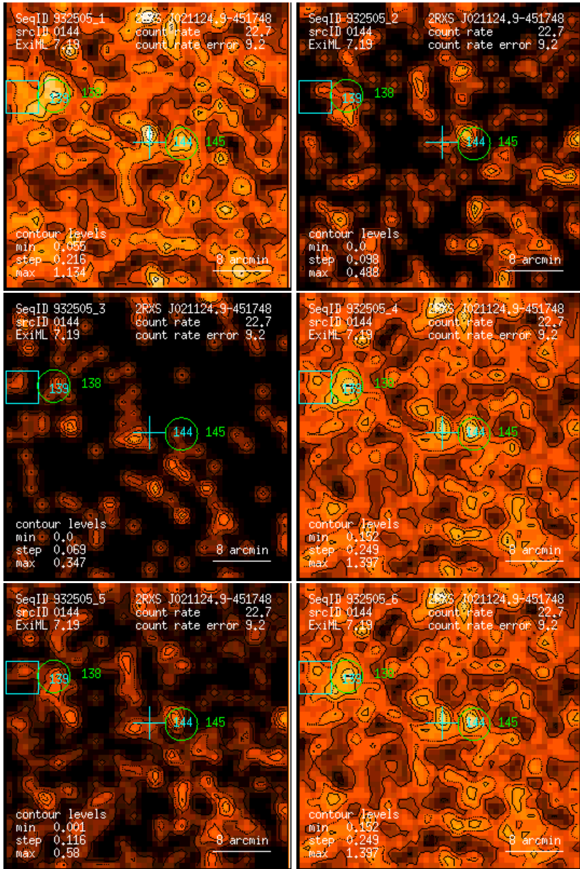
Figure 144: RASS 932505: detection 0144: band rate images, Gaussian filter: (1) PSPC channels 11 – 41, (2) 52 – 90, (3) 91 – 201, (4) 11 – 235, (5) 52 – 201, (6) 11 – 201. Broad band rates in counts/ks. Band rate contour levels in counts/ks/arcmin 2 .
