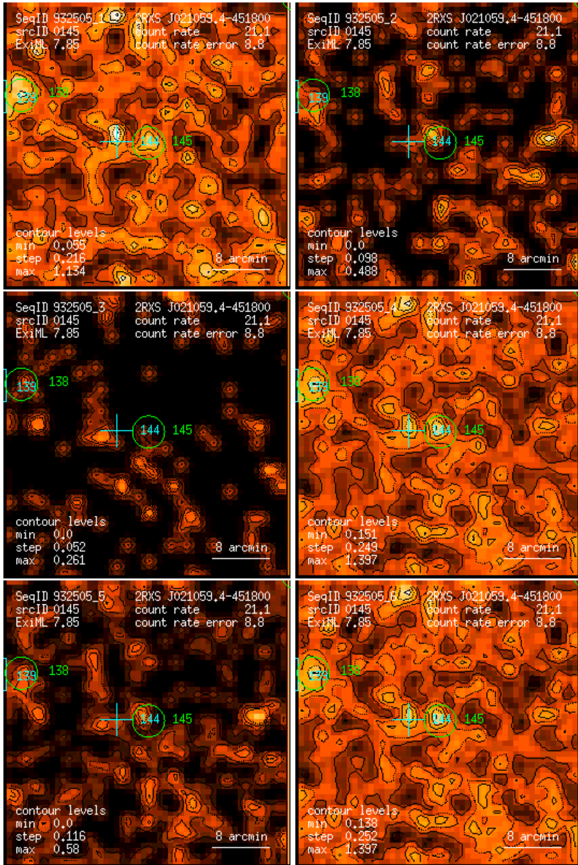
Figure 145: RASS 932505: detection 0145: band rate images, Gaussian filter: (1) PSPC channels 11 – 41, (2) 52 – 90, (3) 91 – 201, (4) 11 – 235, (5) 52 – 201, (6) 11 – 201. Broad band rates in counts/ks. Band rate contour levels in counts/ks/arcmin 2 .
