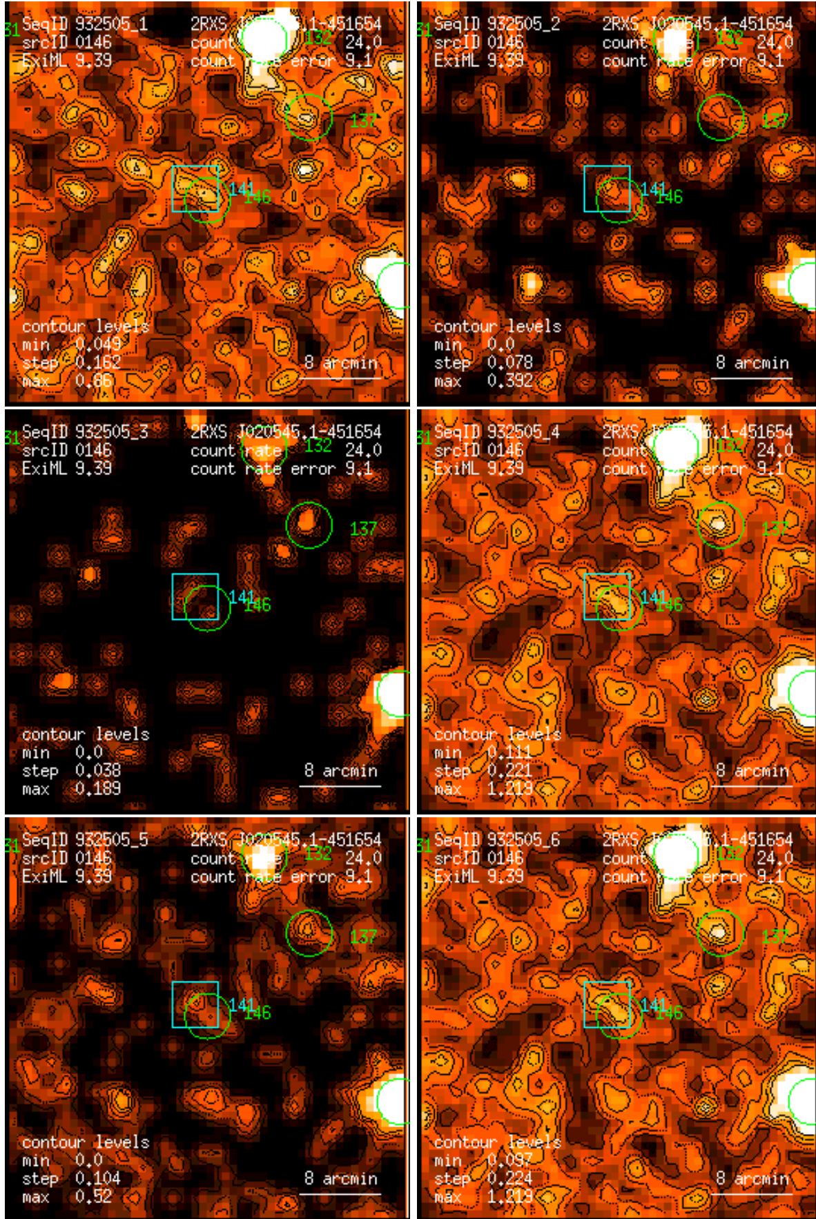
Figure 146: RASS 932505: detection 0146: band rate images, Gaussian filter: (1) PSPC channels 11 – 41, (2) 52 – 90, (3) 91 – 201, (4) 11 – 235, (5) 52 – 201, (6) 11 – 201. Broad band rates in counts/ks. Band rate contour levels in counts/ks/arcmin 2 .
