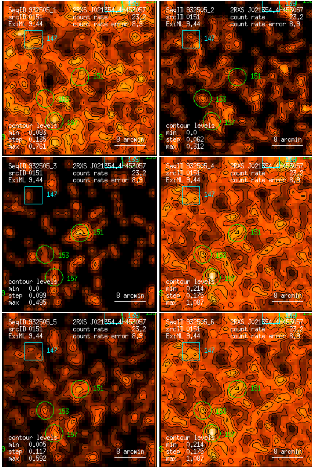
Figure 151: RASS 932505: detection 0151: band rate images, Gaussian filter: (1) PSPC channels 11 – 41, (2) 52 – 90, (3) 91 – 201, (4) 11 – 235, (5) 52 – 201, (6) 11 – 201. Broad band rates in counts/ks. Band rate contour levels in counts/ks/arcmin 2 .
