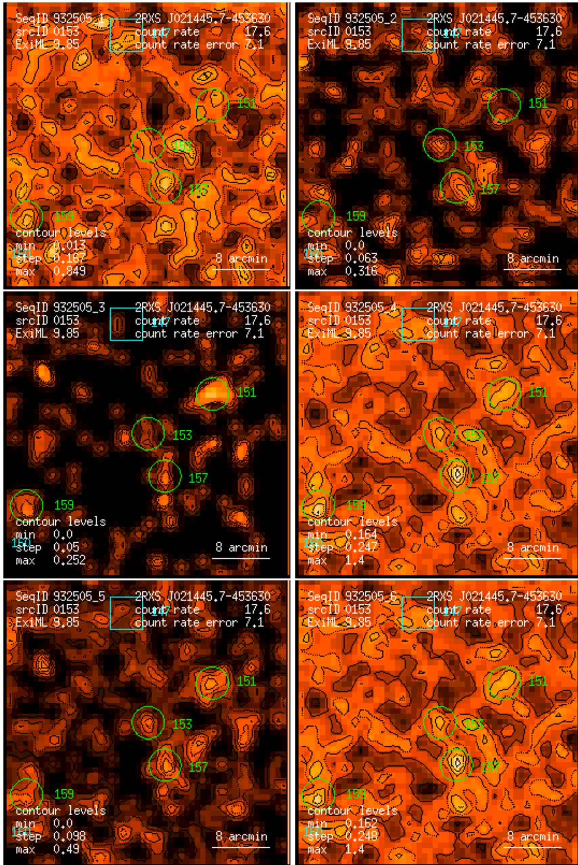
Figure 153: RASS 932505: detection 0153: band rate images, Gaussian filter: (1) PSPC channels 11 – 41, (2) 52 – 90, (3) 91 – 201, (4) 11 – 235, (5) 52 – 201, (6) 11 – 201. Broad band rates in counts/ks. Band rate contour levels in counts/ks/arcmin 2 .
