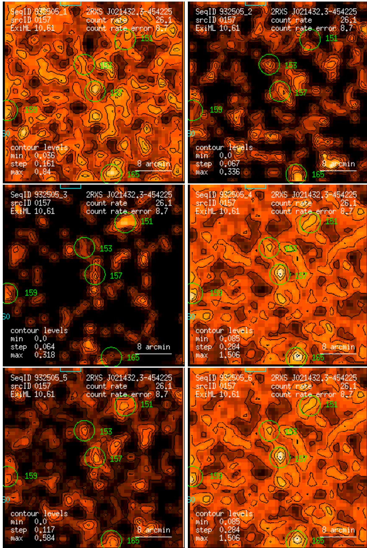
Figure 157: RASS 932505: detection 0157: band rate images, Gaussian filter: (1) PSPC channels 11 – 41, (2) 52 – 90, (3) 91 – 201, (4) 11 – 235, (5) 52 – 201, (6) 11 – 201. Broad band rates in counts/ks. Band rate contour levels in counts/ks/arcmin 2 .
