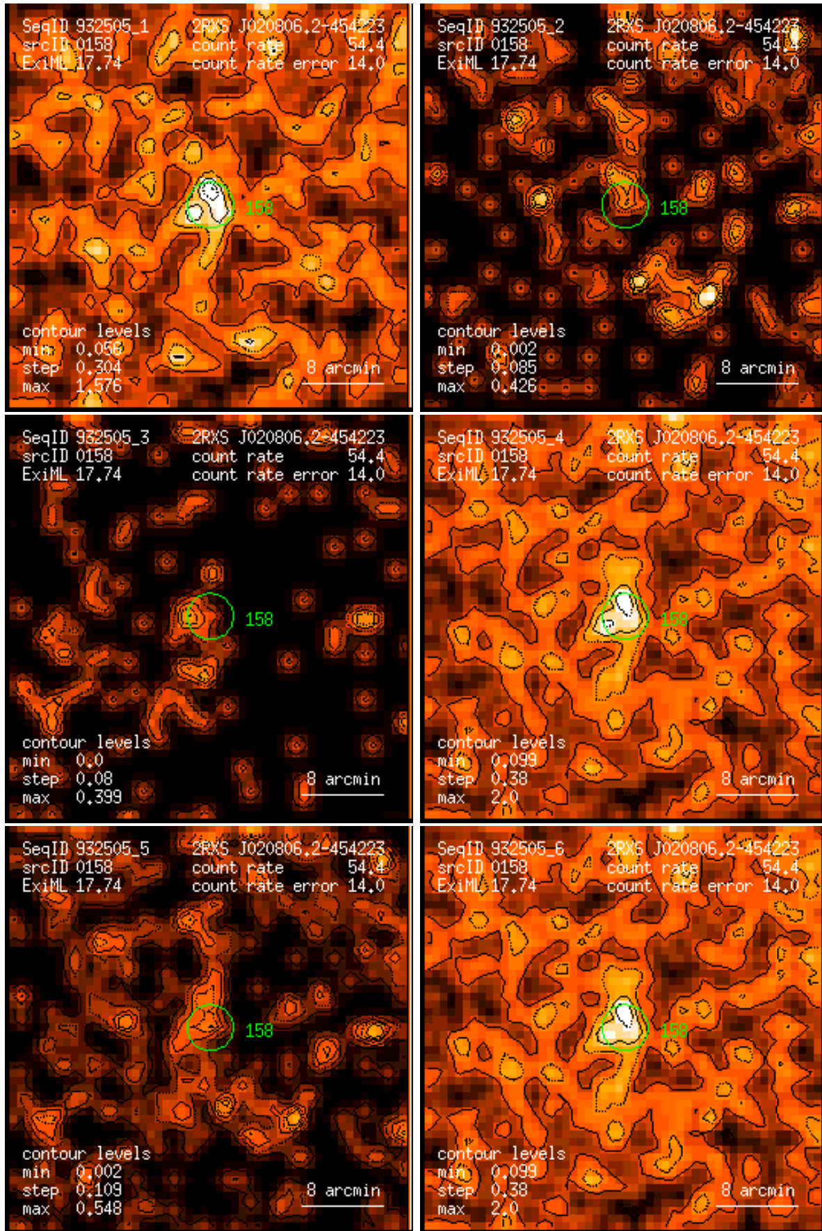
Figure 158: RASS 932505: detection 0158: band rate images, Gaussian filter: (1) PSPC channels 11 – 41, (2) 52 – 90, (3) 91 – 201, (4) 11 – 235, (5) 52 – 201, (6) 11 – 201. Broad band rates in counts/ks. Band rate contour levels in counts/ks/arcmin 2 .
