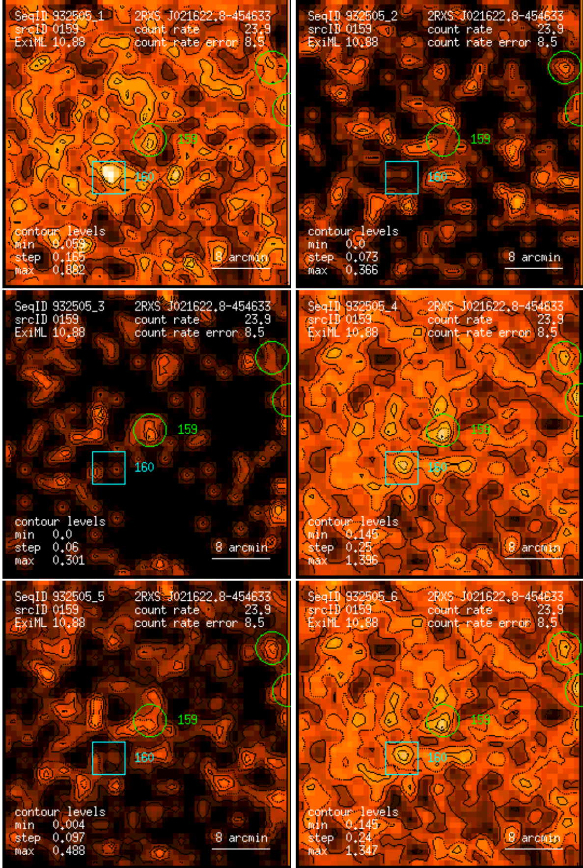
Figure 159: RASS 932505: detection 0159: band rate images, Gaussian filter: (1) PSPC channels 11 – 41, (2) 52 – 90, (3) 91 – 201, (4) 11 – 235, (5) 52 – 201, (6) 11 – 201. Broad band rates in counts/ks. Band rate contour levels in counts/ks/arcmin 2 .
