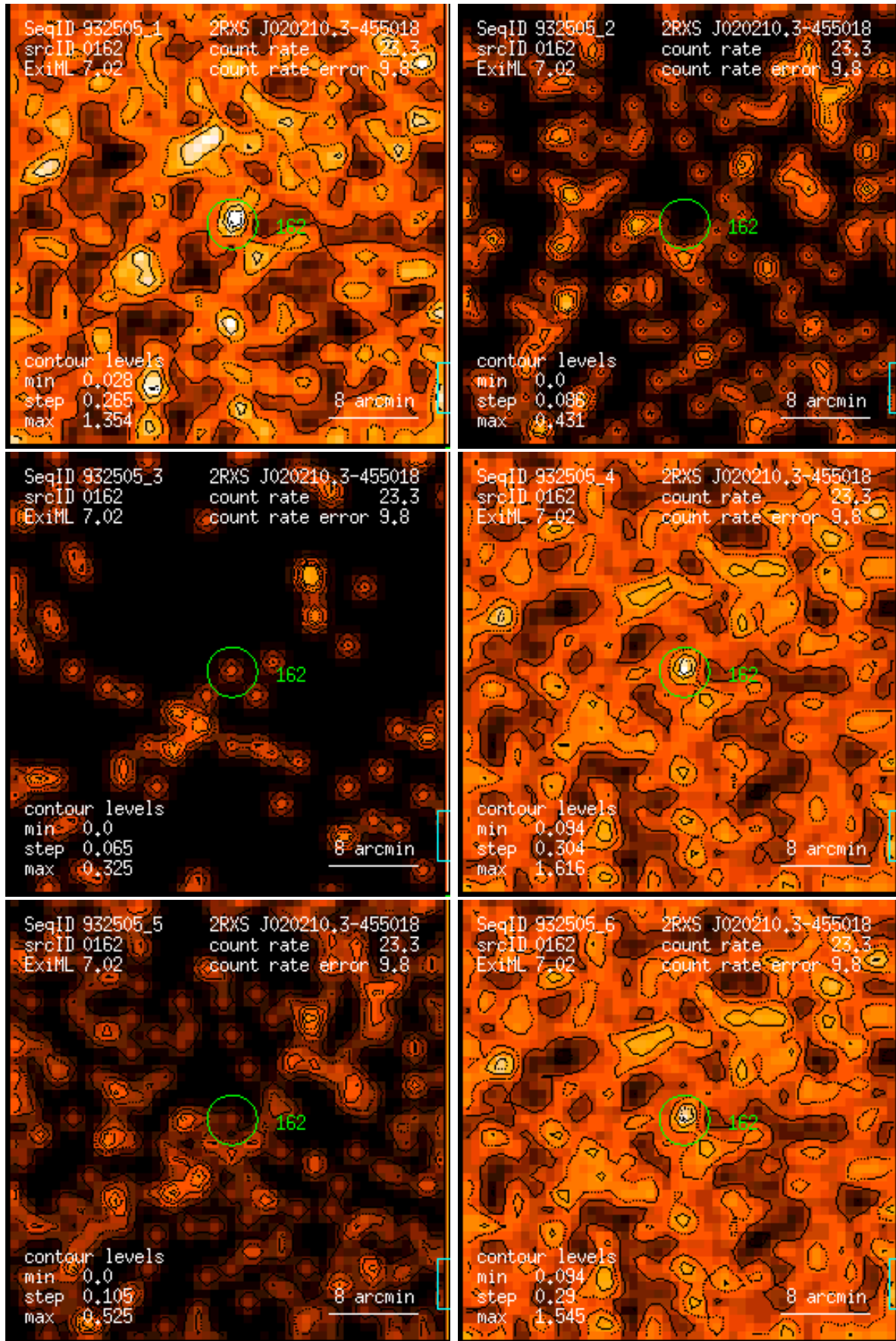
Figure 162: RASS 932505: detection 0162: band rate images, Gaussian filter: (1) PSPC channels 11 – 41, (2) 52 – 90, (3) 91 – 201, (4) 11 – 235, (5) 52 – 201, (6) 11 – 201. Broad band rates in counts/ks. Band rate contour levels in counts/ks/arcmin 2 .
