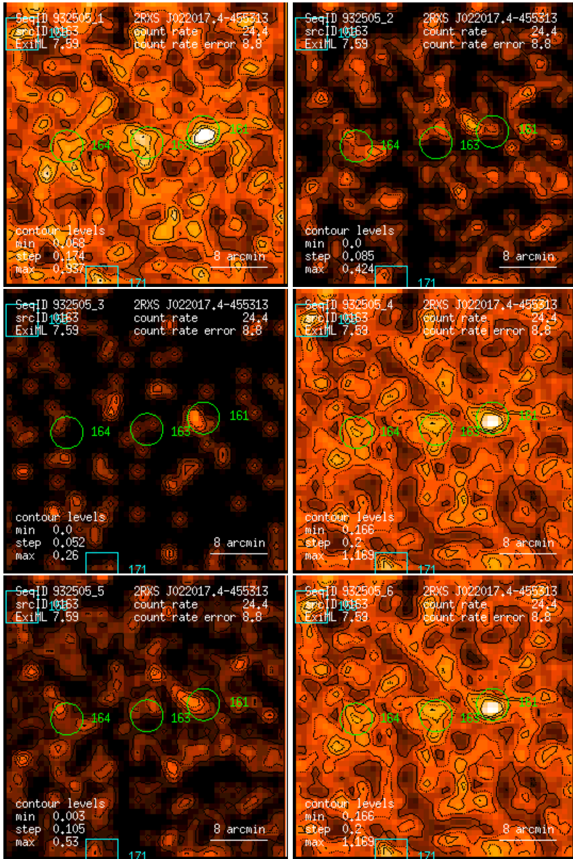
Figure 163: RASS 932505: detection 0163: band rate images, Gaussian filter: (1) PSPC channels 11 – 41, (2) 52 – 90, (3) 91 – 201, (4) 11 – 235, (5) 52 – 201, (6) 11 – 201. Broad band rates in counts/ks. Band rate contour levels in counts/ks/arcmin 2 .
