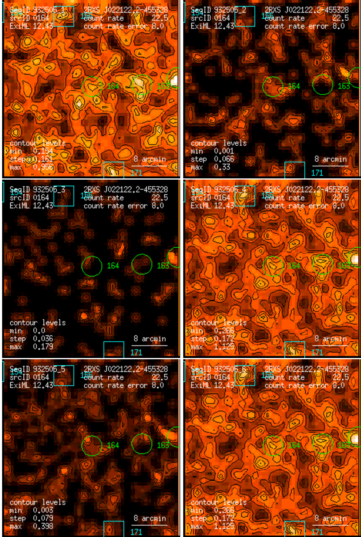
Figure 164: RASS 932505: detection 0164: band rate images, Gaussian filter: (1) PSPC channels 11 – 41, (2) 52 – 90, (3) 91 – 201, (4) 11 – 235, (5) 52 – 201, (6) 11 – 201. Broad band rates in counts/ks. Band rate contour levels in counts/ks/arcmin 2 .
