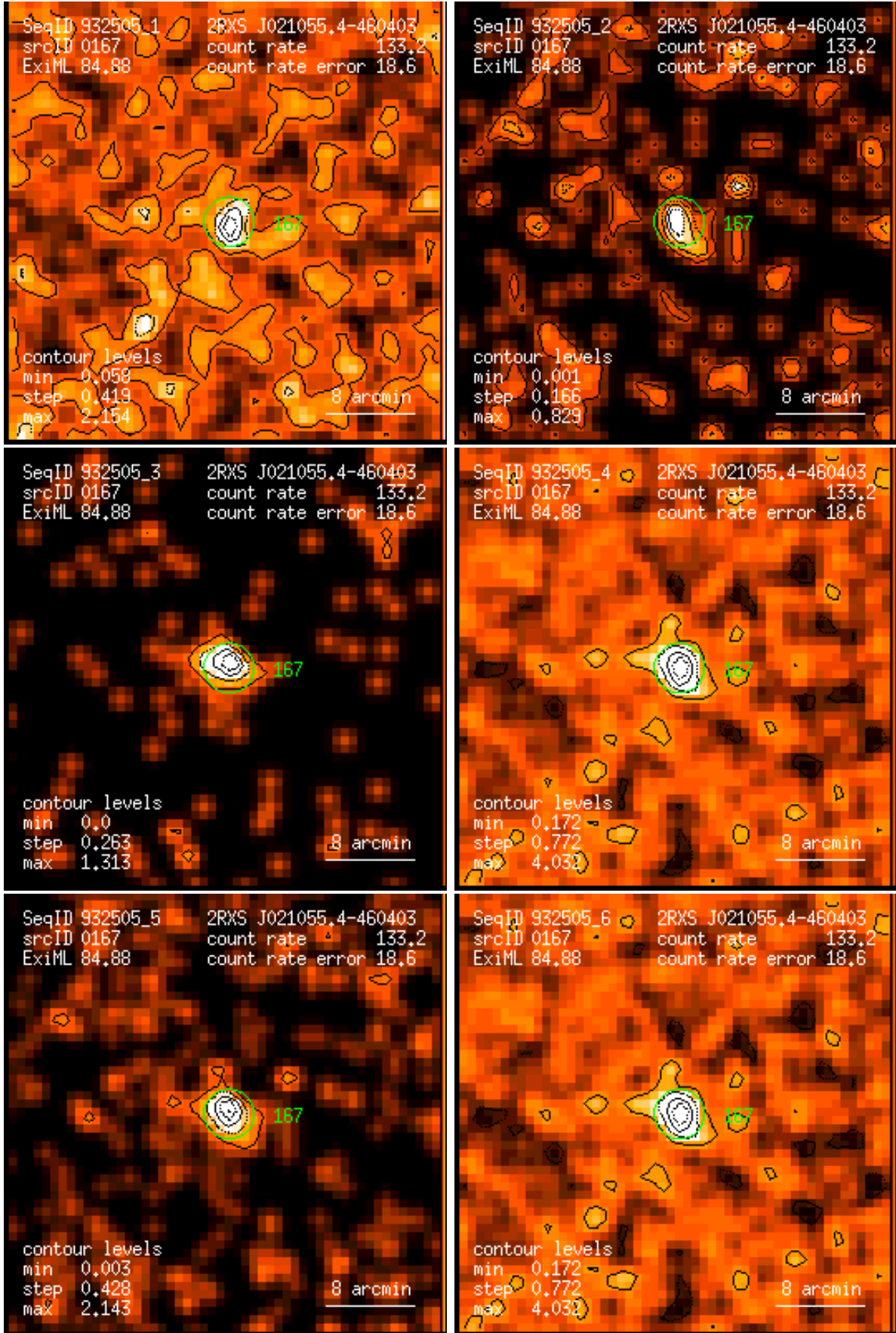
Figure 167: RASS 932505: detection 0167: band rate images, Gaussian filter: (1) PSPC channels 11 – 41, (2) 52 – 90, (3) 91 – 201, (4) 11 – 235, (5) 52 – 201, (6) 11 – 201. Broad band rates in counts/ks. Band rate contour levels in counts/ks/arcmin 2 .
