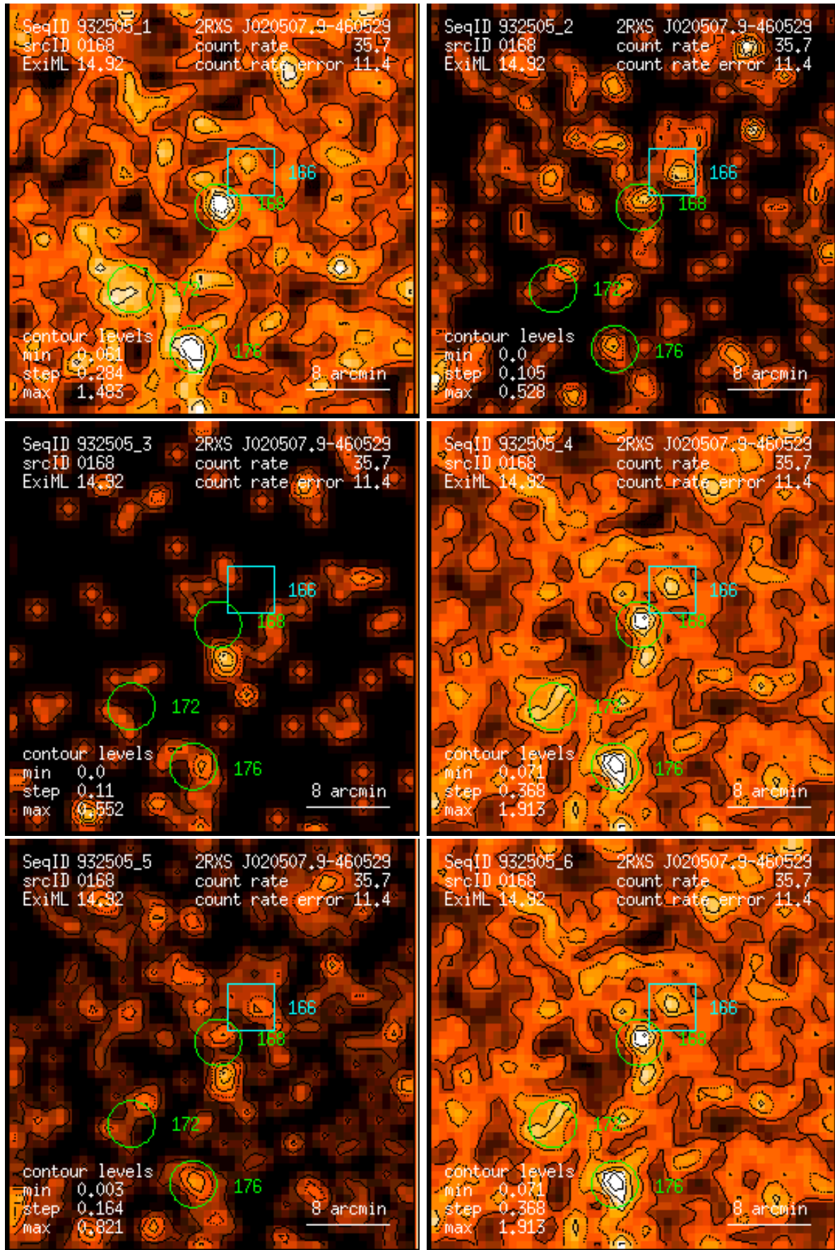
Figure 168: RASS 932505: detection 0168: band rate images, Gaussian filter: (1) PSPC channels 11 – 41, (2) 52 – 90, (3) 91 – 201, (4) 11 – 235, (5) 52 – 201, (6) 11 – 201. Broad band rates in counts/ks. Band rate contour levels in counts/ks/arcmin 2 .
