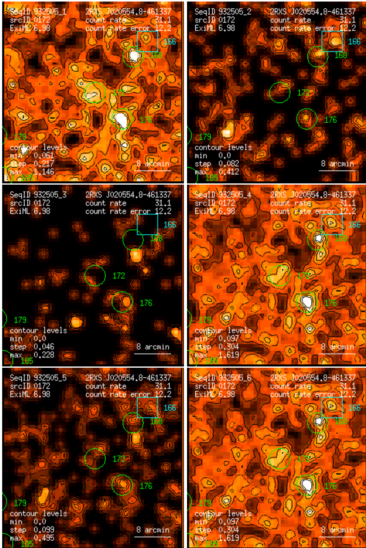
Figure 172: RASS 932505: detection 0172: band rate images, Gaussian filter: (1) PSPC channels 11 – 41, (2) 52 – 90, (3) 91 – 201, (4) 11 – 235, (5) 52 – 201, (6) 11 – 201. Broad band rates in counts/ks. Band rate contour levels in counts/ks/arcmin 2 .
