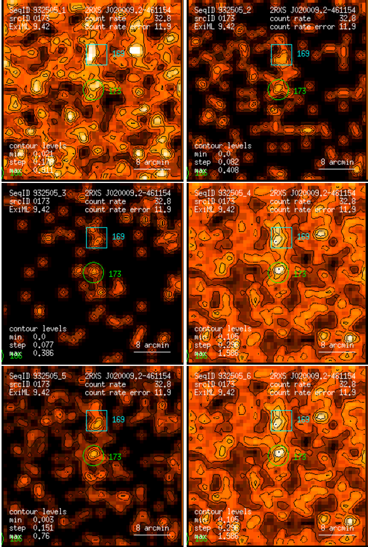
Figure 173: RASS 932505: detection 0173: band rate images, Gaussian filter: (1) PSPC channels 11 – 41, (2) 52 – 90, (3) 91 – 201, (4) 11 – 235, (5) 52 – 201, (6) 11 – 201. Broad band rates in counts/ks. Band rate contour levels in counts/ks/arcmin 2 .
