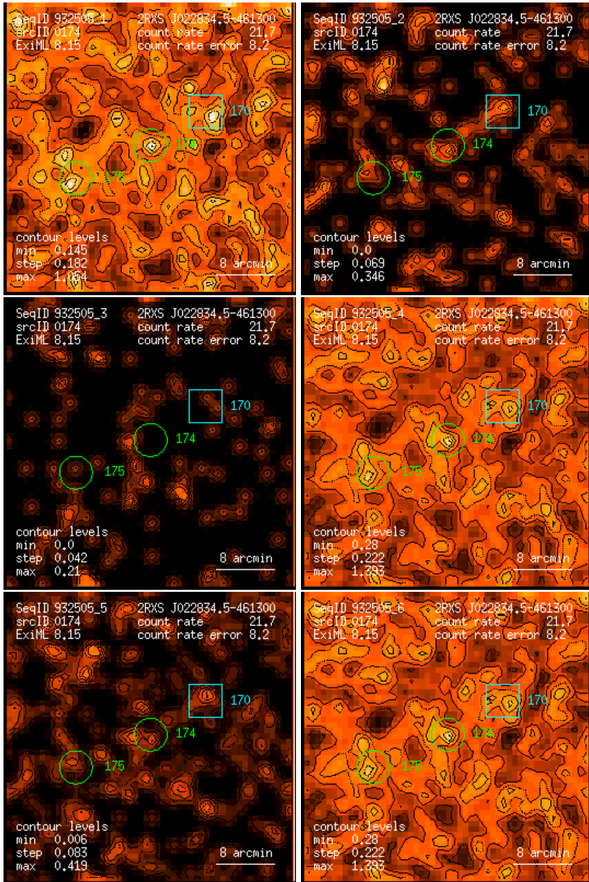
Figure 174: RASS 932505: detection 0174: band rate images, Gaussian filter: (1) PSPC channels 11 – 41, (2) 52 – 90, (3) 91 – 201, (4) 11 – 235, (5) 52 – 201, (6) 11 – 201. Broad band rates in counts/ks. Band rate contour levels in counts/ks/arcmin 2 .
