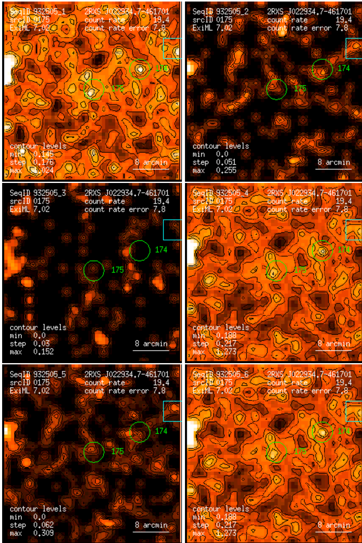
Figure 175: RASS 932505: detection 0175: band rate images, Gaussian filter: (1) PSPC channels 11 – 41, (2) 52 – 90, (3) 91 – 201, (4) 11 – 235, (5) 52 – 201, (6) 11 – 201. Broad band rates in counts/ks. Band rate contour levels in counts/ks/arcmin 2 .
