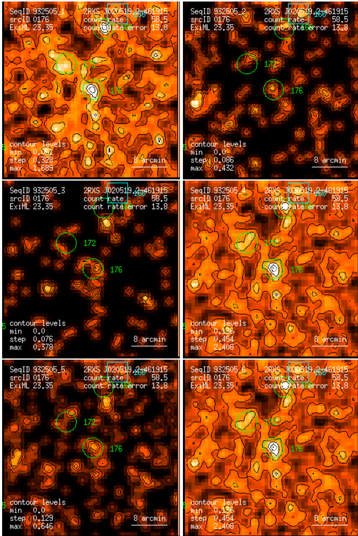
Figure 176: RASS 932505: detection 0176: band rate images, Gaussian filter: (1) PSPC channels 11 – 41, (2) 52 – 90, (3) 91 – 201, (4) 11 – 235, (5) 52 – 201, (6) 11 – 201. Broad band rates in counts/ks. Band rate contour levels in counts/ks/arcmin 2 .
