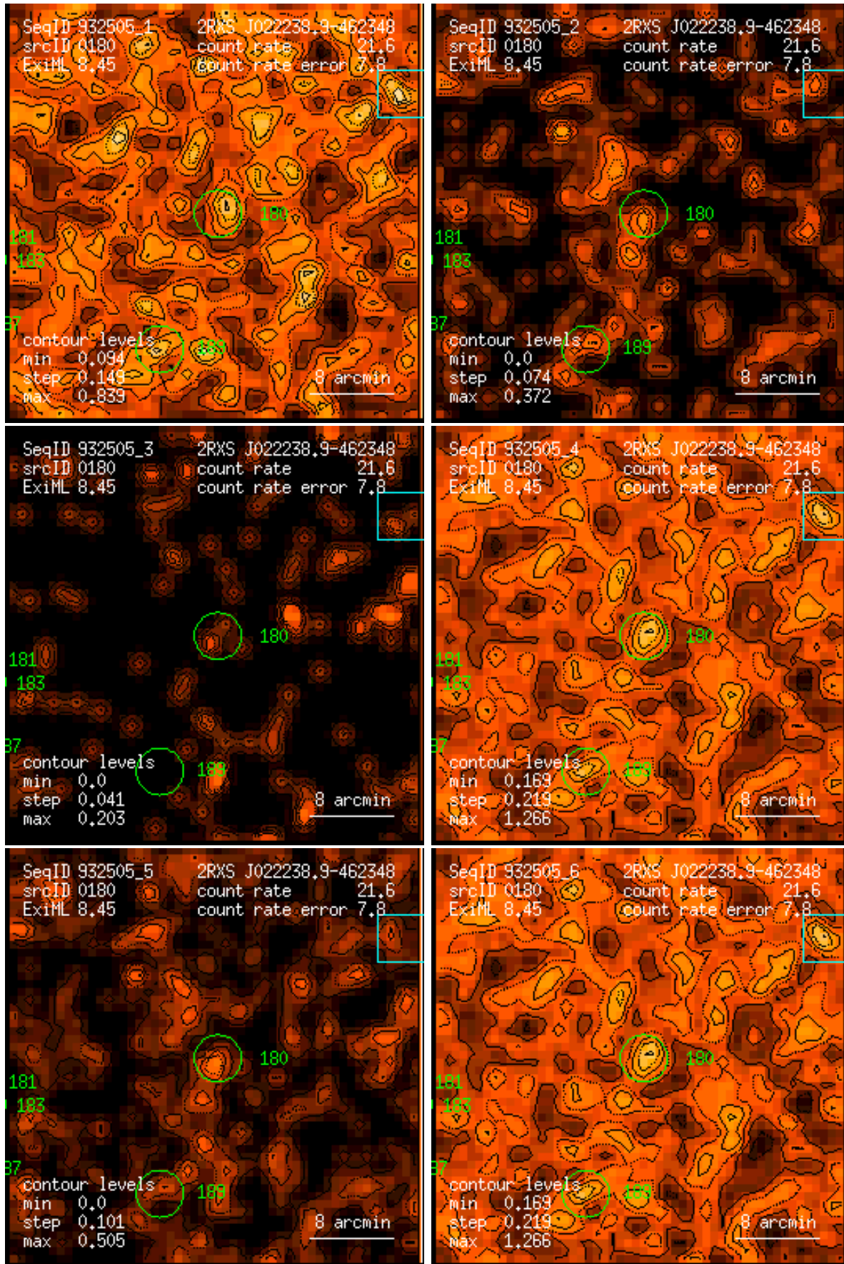
Figure 180: RASS 932505: detection 0180: band rate images, Gaussian filter: (1) PSPC channels 11 – 41, (2) 52 – 90, (3) 91 – 201, (4) 11 – 235, (5) 52 – 201, (6) 11 – 201. Broad band rates in counts/ks. Band rate contour levels in counts/ks/arcmin 2 .
