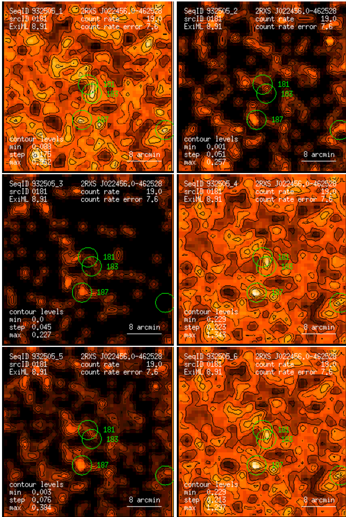
Figure 181: RASS 932505: detection 0181: band rate images, Gaussian filter: (1) PSPC channels 11 – 41, (2) 52 – 90, (3) 91 – 201, (4) 11 – 235, (5) 52 – 201, (6) 11 – 201. Broad band rates in counts/ks. Band rate contour levels in counts/ks/arcmin 2 .
