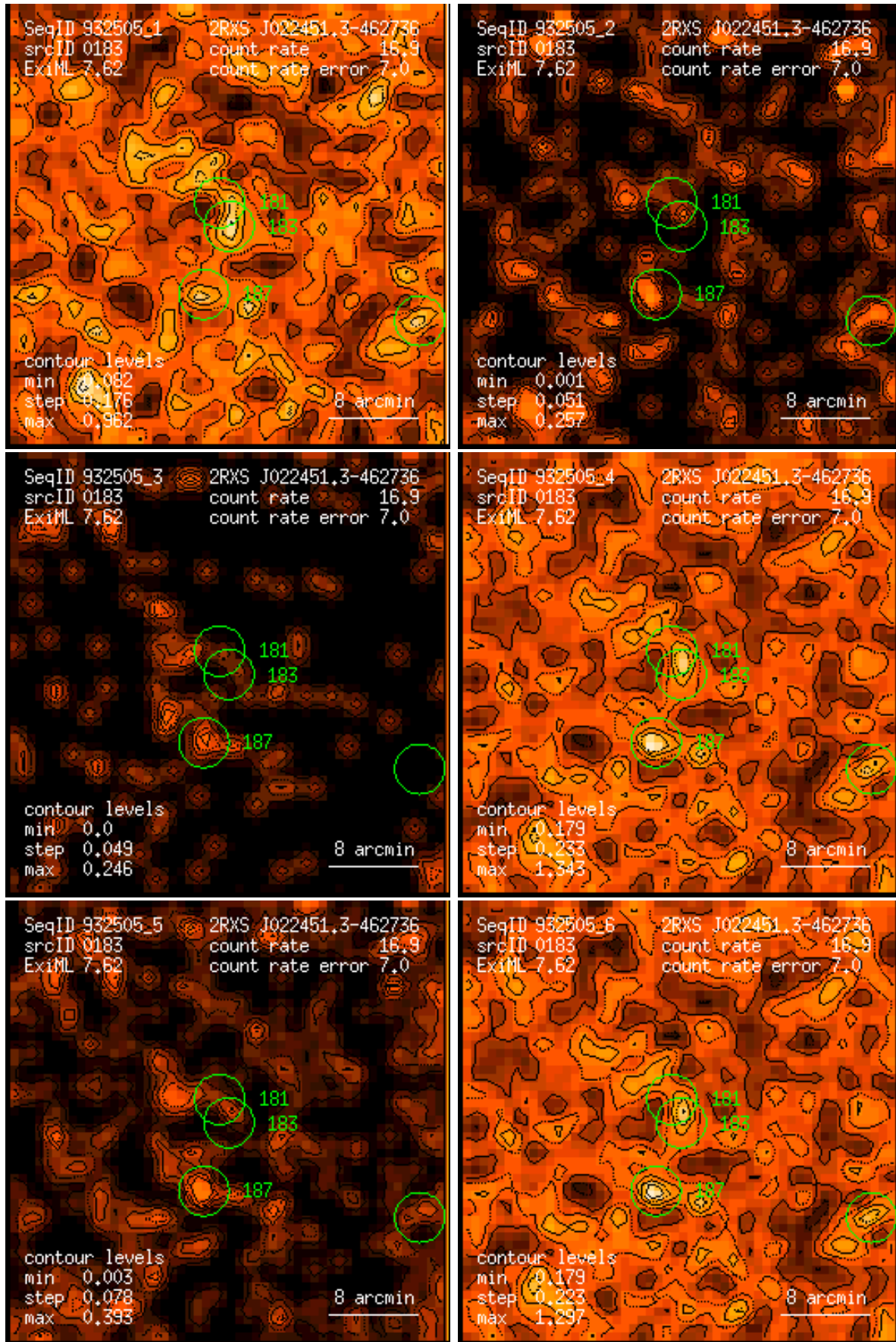
Figure 183: RASS 932505: detection 0183: band rate images, Gaussian filter: (1) PSPC channels 11 – 41, (2) 52 – 90, (3) 91 – 201, (4) 11 – 235, (5) 52 – 201, (6) 11 – 201. Broad band rates in counts/ks. Band rate contour levels in counts/ks/arcmin 2 .
