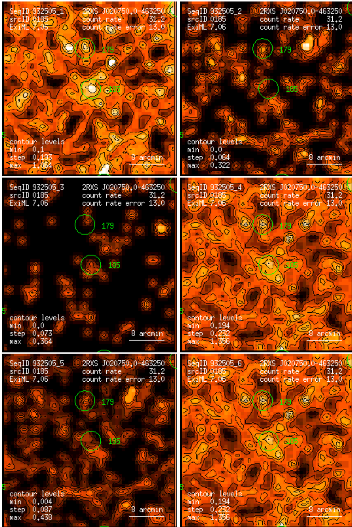
Figure 185: RASS 932505: detection 0185: band rate images, Gaussian filter: (1) PSPC channels 11 – 41, (2) 52 – 90, (3) 91 – 201, (4) 11 – 235, (5) 52 – 201, (6) 11 – 201. Broad band rates in counts/ks. Band rate contour levels in counts/ks/arcmin 2 .
