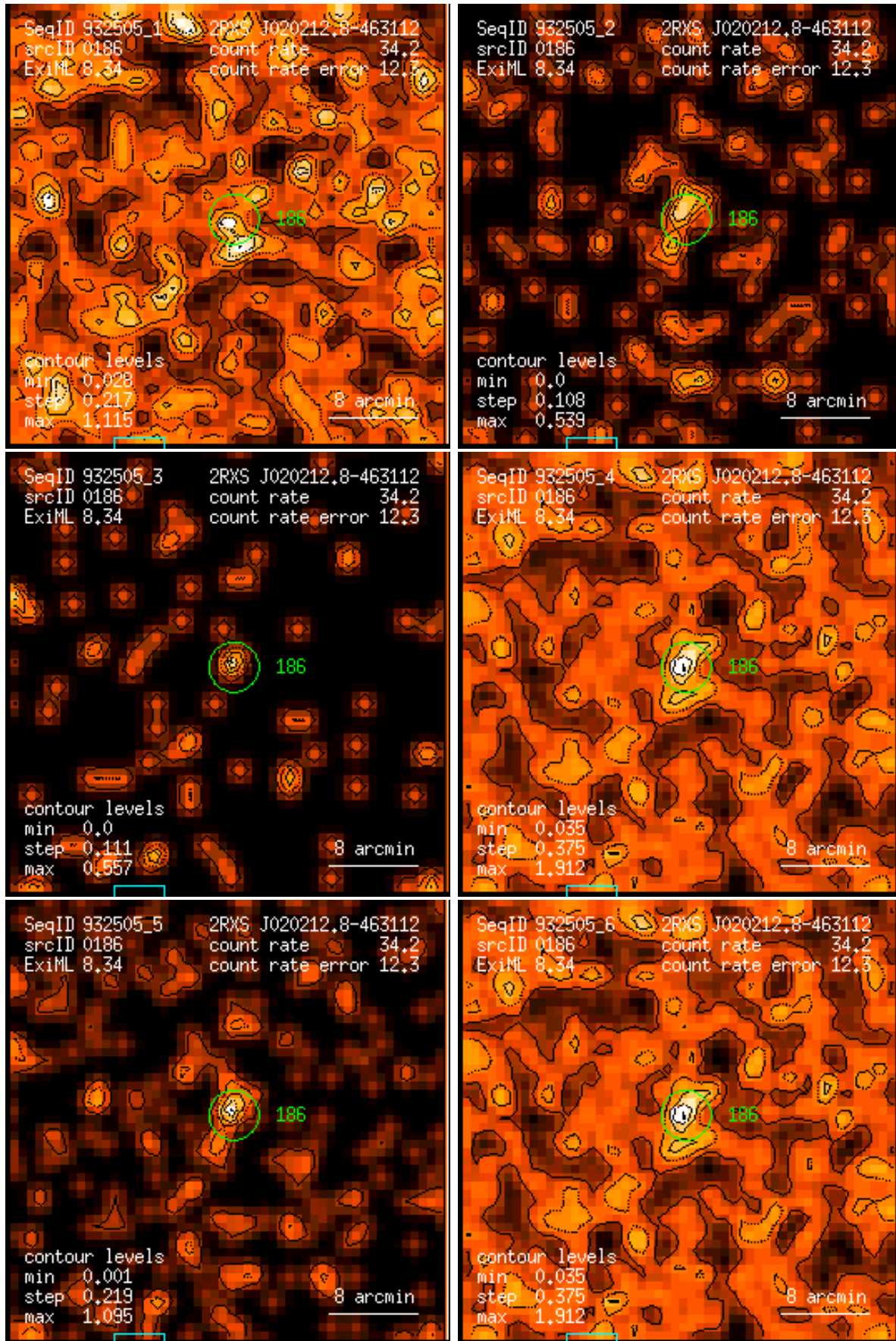
Figure 186: RASS 932505: detection 0186: band rate images, Gaussian filter: (1) PSPC channels 11 – 41, (2) 52 – 90, (3) 91 – 201, (4) 11 – 235, (5) 52 – 201, (6) 11 – 201. Broad band rates in counts/ks. Band rate contour levels in counts/ks/arcmin 2 .
