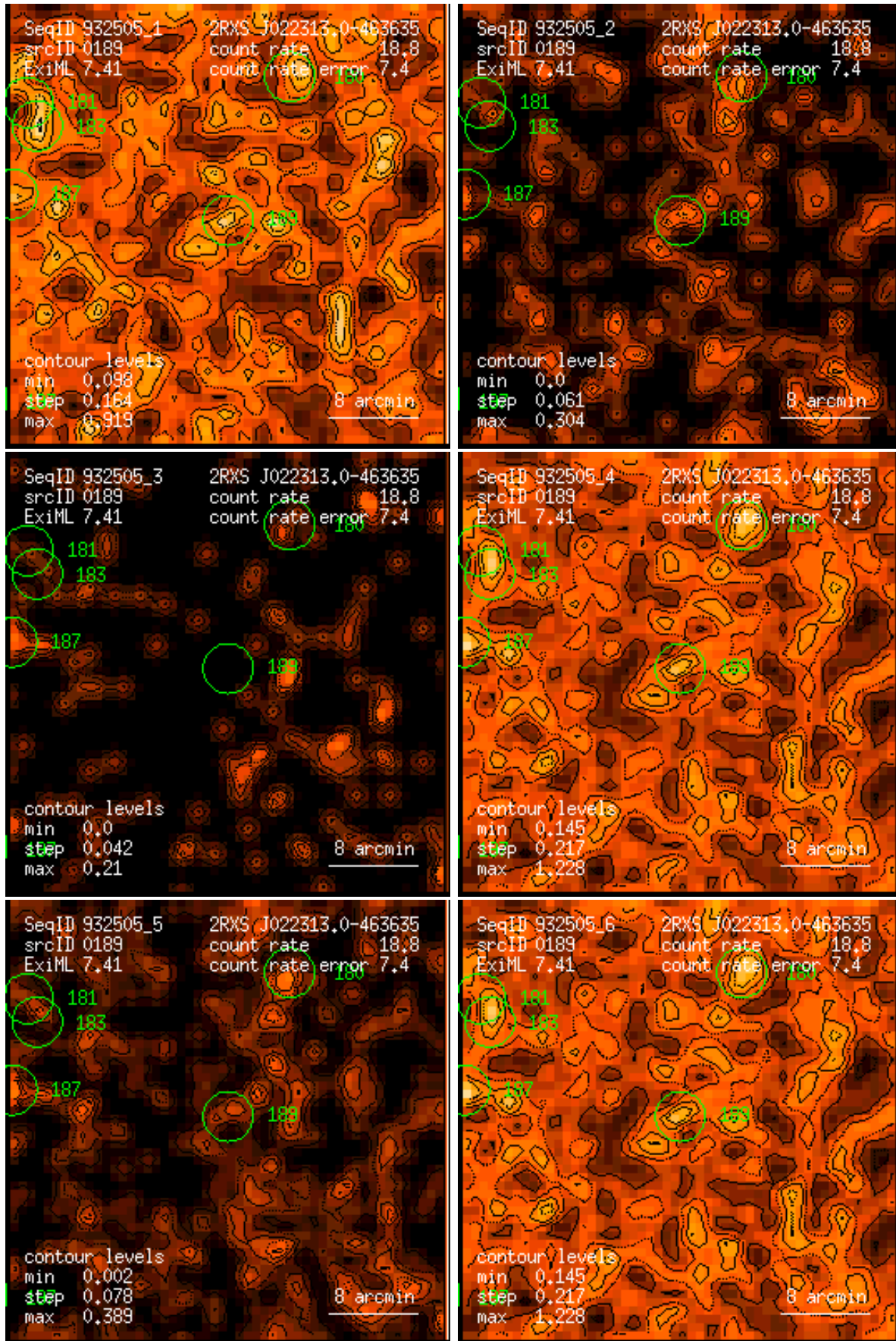
Figure 189: RASS 932505: detection 0189: band rate images, Gaussian filter: (1) PSPC channels 11 – 41, (2) 52 – 90, (3) 91 – 201, (4) 11 – 235, (5) 52 – 201, (6) 11 – 201. Broad band rates in counts/ks. Band rate contour levels in counts/ks/arcmin 2 .
