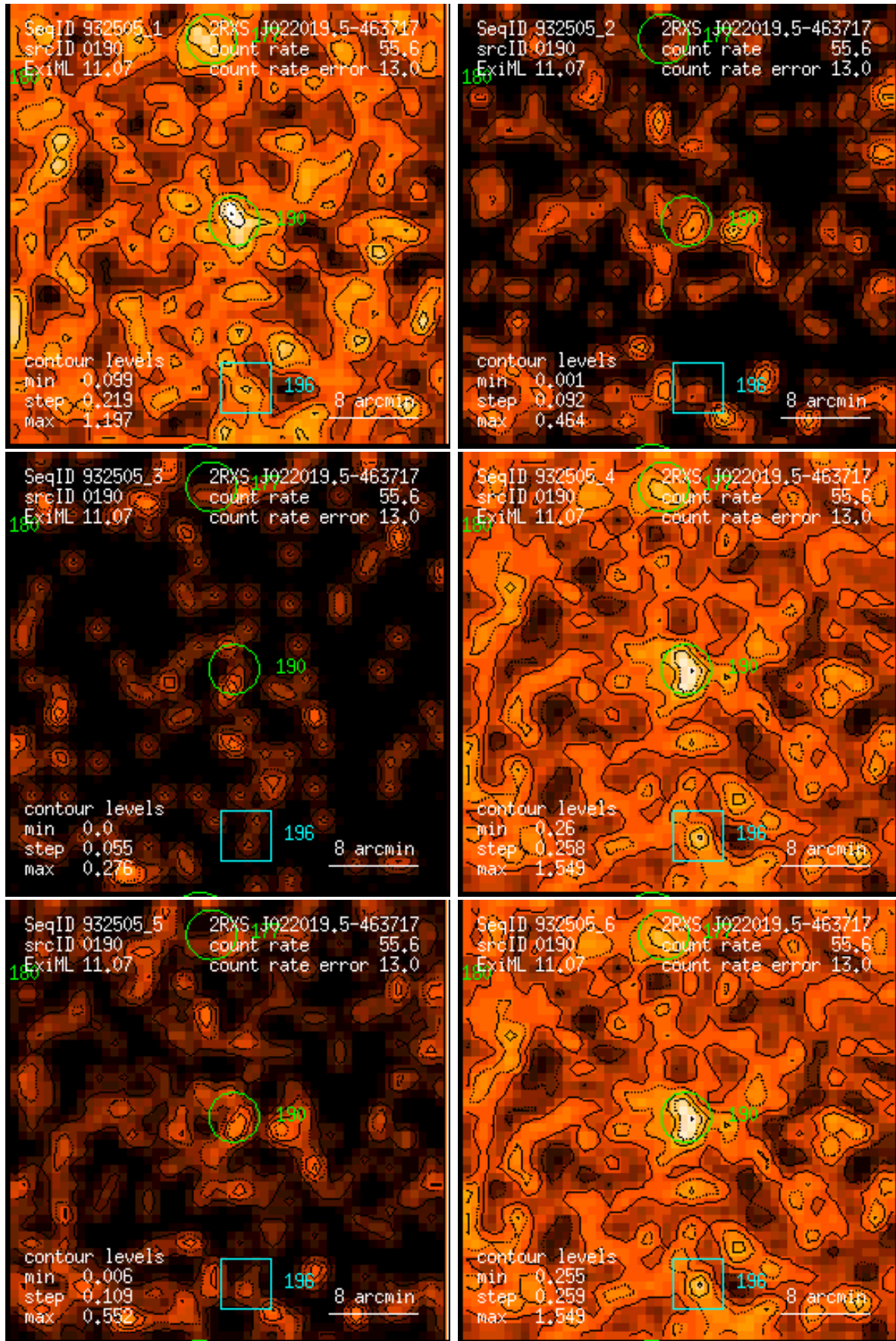
Figure 190: RASS 932505: detection 0190: band rate images, Gaussian filter: (1) PSPC channels 11 – 41, (2) 52 – 90, (3) 91 – 201, (4) 11 – 235, (5) 52 – 201, (6) 11 – 201. Broad band rates in counts/ks. Band rate contour levels in counts/ks/arcmin 2 .
