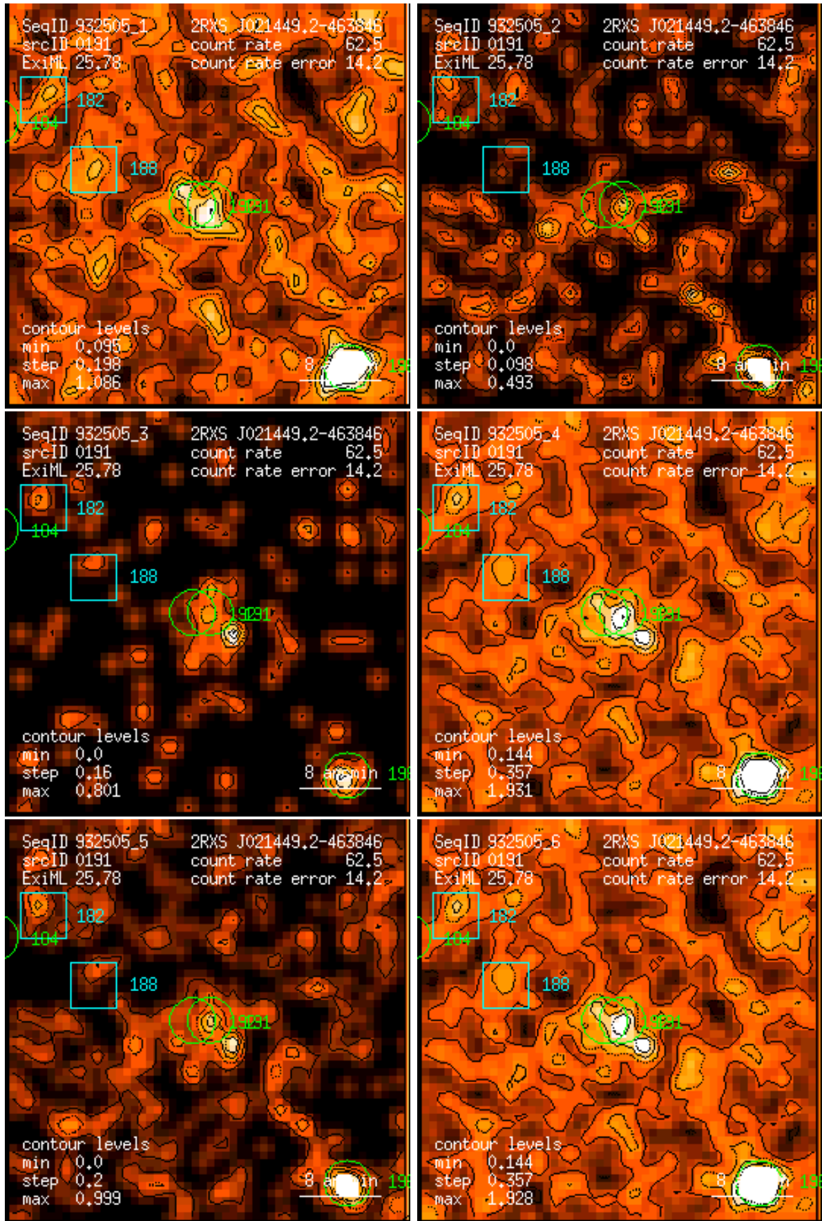
Figure 191: RASS 932505: detection 0191: band rate images, Gaussian filter: (1) PSPC channels 11 – 41, (2) 52 – 90, (3) 91 – 201, (4) 11 – 235, (5) 52 – 201, (6) 11 – 201. Broad band rates in counts/ks. Band rate contour levels in counts/ks/arcmin 2 .
