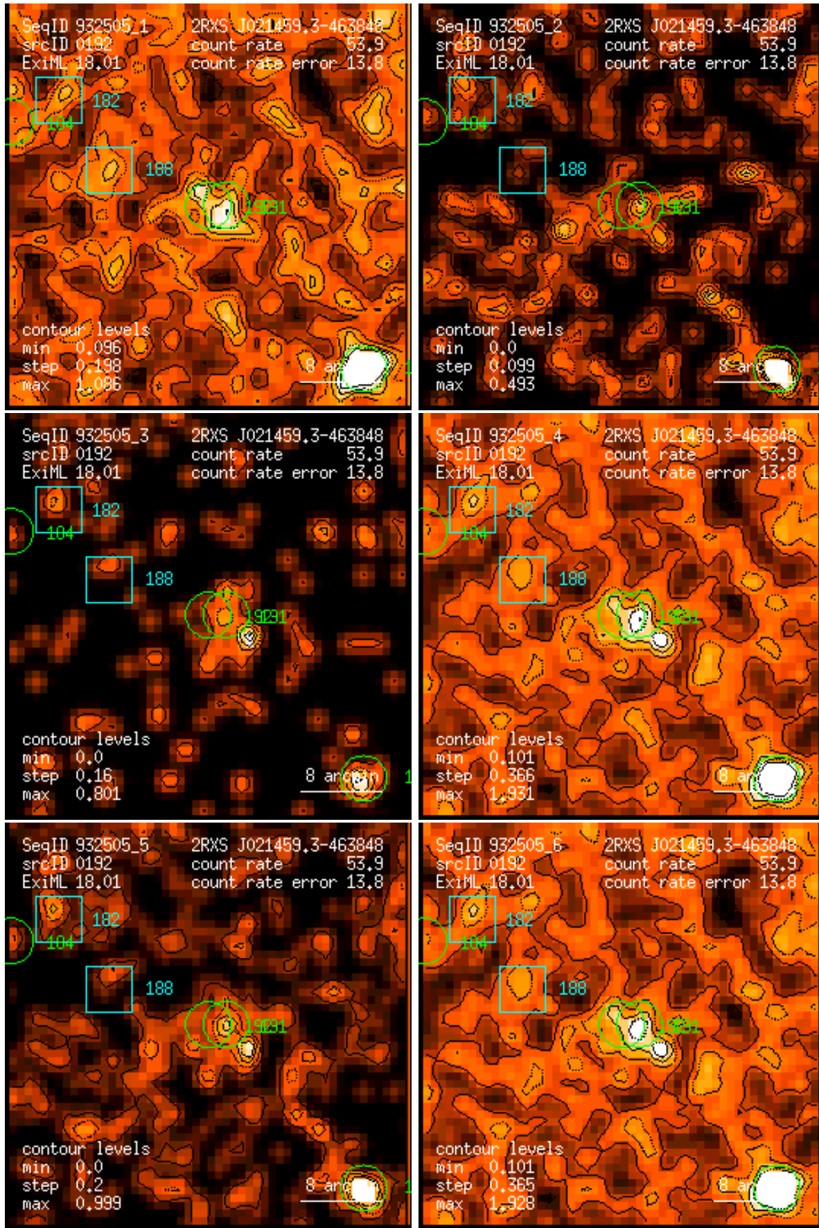
Figure 192: RASS 932505: detection 0192: band rate images, Gaussian filter: (1) PSPC channels 11 – 41, (2) 52 – 90, (3) 91 – 201, (4) 11 – 235, (5) 52 – 201, (6) 11 – 201. Broad band rates in counts/ks. Band rate contour levels in counts/ks/arcmin 2 .
