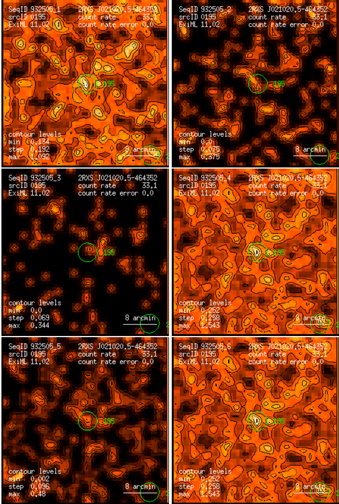
Figure 195: RASS 932505: detection 0195: band rate images, Gaussian filter: (1) PSPC channels 11 – 41, (2) 52 – 90, (3) 91 – 201, (4) 11 – 235, (5) 52 – 201, (6) 11 – 201. Broad band rates in counts/ks. Band rate contour levels in counts/ks/arcmin 2 .
