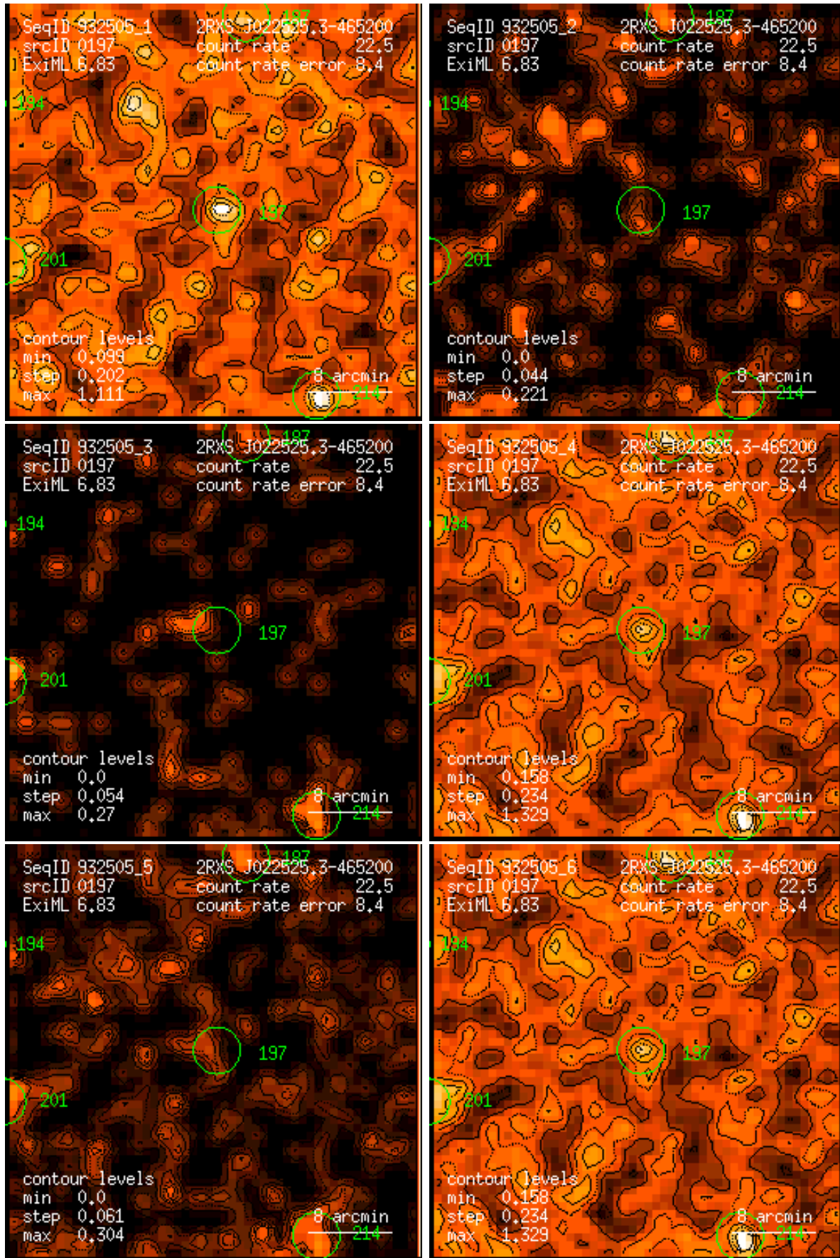
Figure 197: RASS 932505: detection 0197: band rate images, Gaussian filter: (1) PSPC channels 11 – 41, (2) 52 – 90, (3) 91 – 201, (4) 11 – 235, (5) 52 – 201, (6) 11 – 201. Broad band rates in counts/ks. Band rate contour levels in counts/ks/arcmin 2 .
