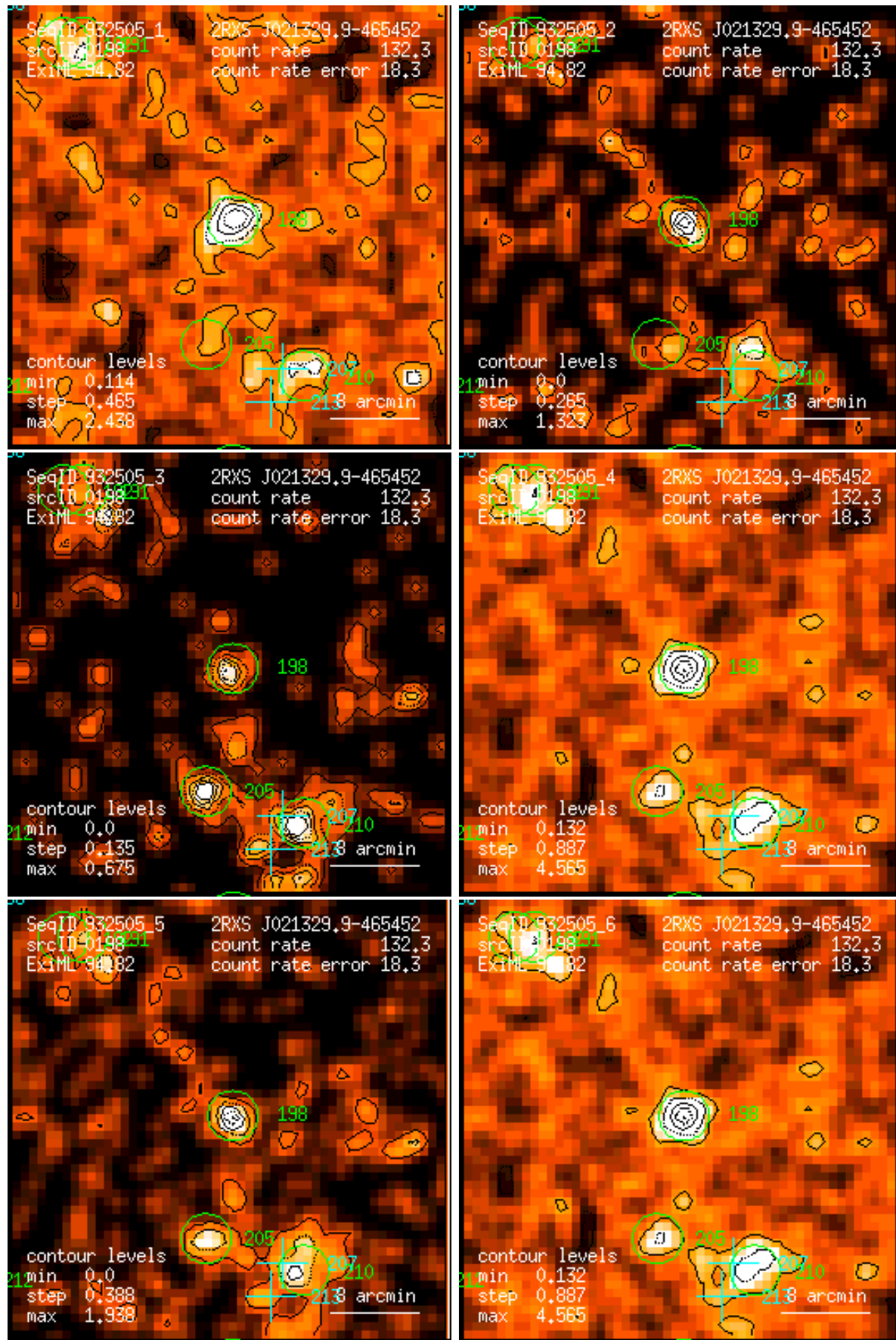
Figure 198: RASS 932505: detection 0198: band rate images, Gaussian filter: (1) PSPC channels 11 – 41, (2) 52 – 90, (3) 91 – 201, (4) 11 – 235, (5) 52 – 201, (6) 11 – 201. Broad band rates in counts/ks. Band rate contour levels in counts/ks/arcmin 2 .
