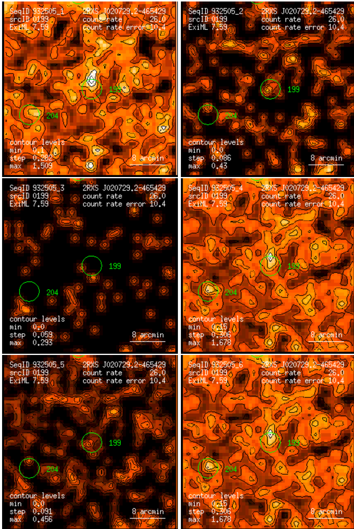
Figure 199: RASS 932505: detection 0199: band rate images, Gaussian filter: (1) PSPC channels 11 – 41, (2) 52 – 90, (3) 91 – 201, (4) 11 – 235, (5) 52 – 201, (6) 11 – 201. Broad band rates in counts/ks. Band rate contour levels in counts/ks/arcmin 2 .
