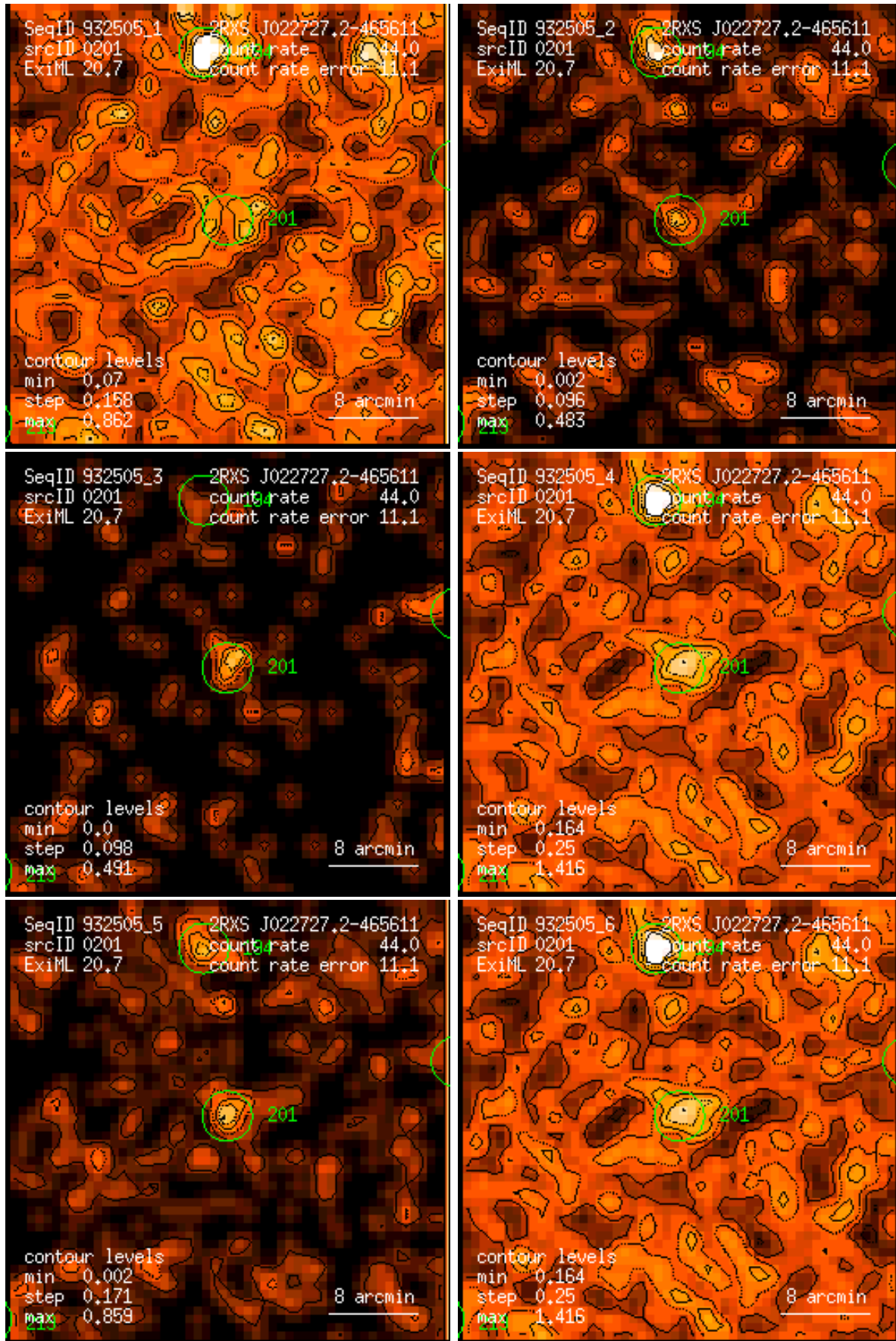
Figure 201: RASS 932505: detection 0201: band rate images, Gaussian filter: (1) PSPC channels 11 – 41, (2) 52 – 90, (3) 91 – 201, (4) 11 – 235, (5) 52 – 201, (6) 11 – 201. Broad band rates in counts/ks. Band rate contour levels in counts/ks/arcmin 2 .
