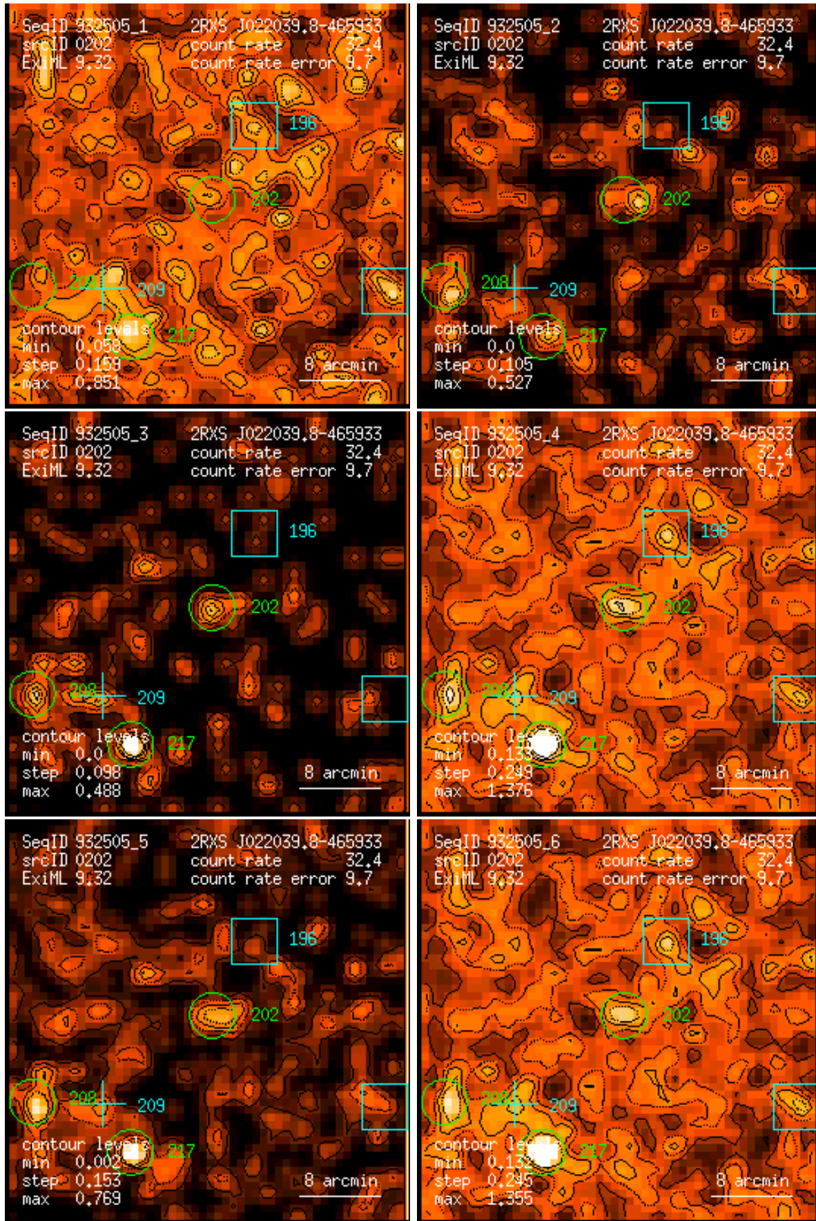
Figure 202: RASS 932505: detection 0202: band rate images, Gaussian filter: (1) PSPC channels 11 – 41, (2) 52 – 90, (3) 91 – 201, (4) 11 – 235, (5) 52 – 201, (6) 11 – 201. Broad band rates in counts/ks. Band rate contour levels in counts/ks/arcmin 2 .
