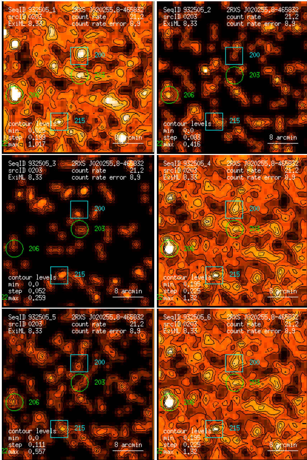
Figure 203: RASS 932505: detection 0203: band rate images, Gaussian filter: (1) PSPC channels 11 – 41, (2) 52 – 90, (3) 91 – 201, (4) 11 – 235, (5) 52 – 201, (6) 11 – 201. Broad band rates in counts/ks. Band rate contour levels in counts/ks/arcmin 2 .
