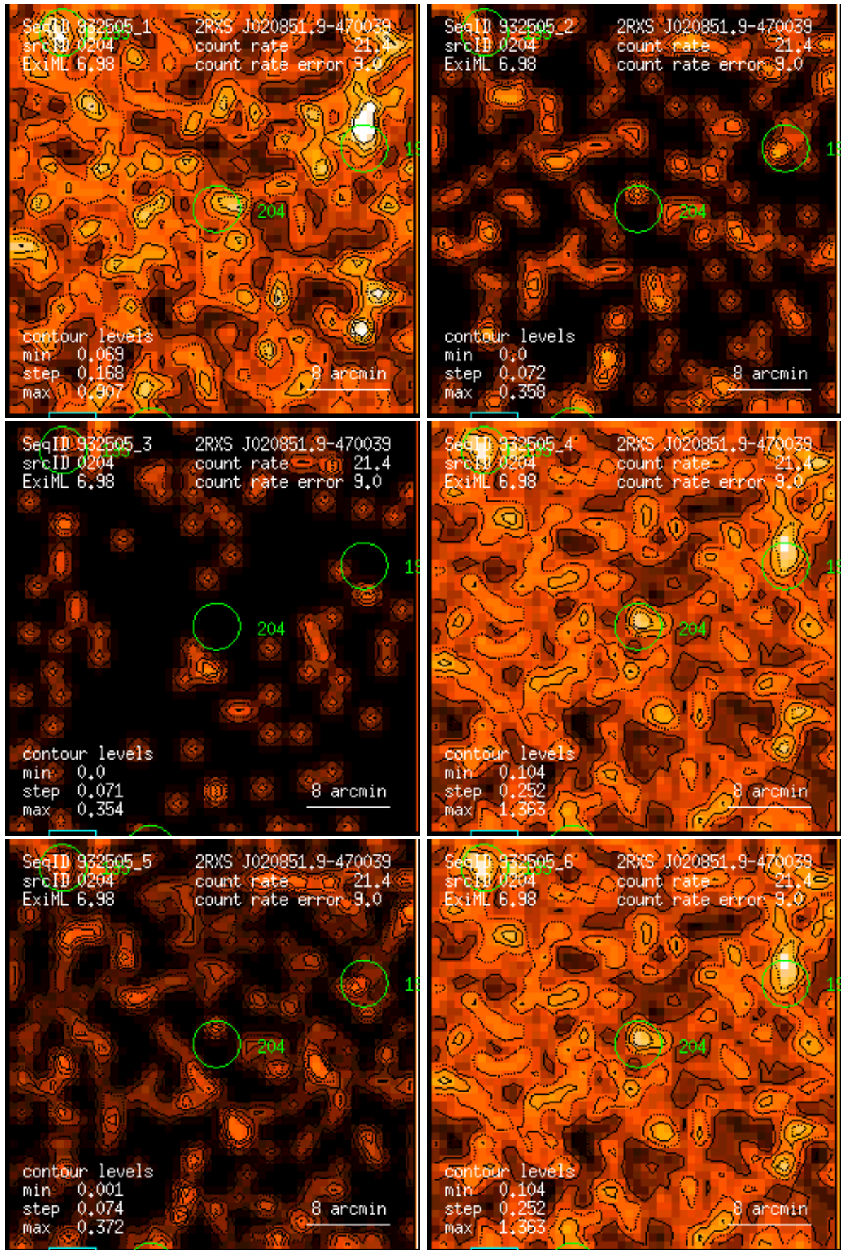
Figure 204: RASS 932505: detection 0204: band rate images, Gaussian filter: (1) PSPC channels 11 – 41, (2) 52 – 90, (3) 91 – 201, (4) 11 – 235, (5) 52 – 201, (6) 11 – 201. Broad band rates in counts/ks. Band rate contour levels in counts/ks/arcmin 2 .
