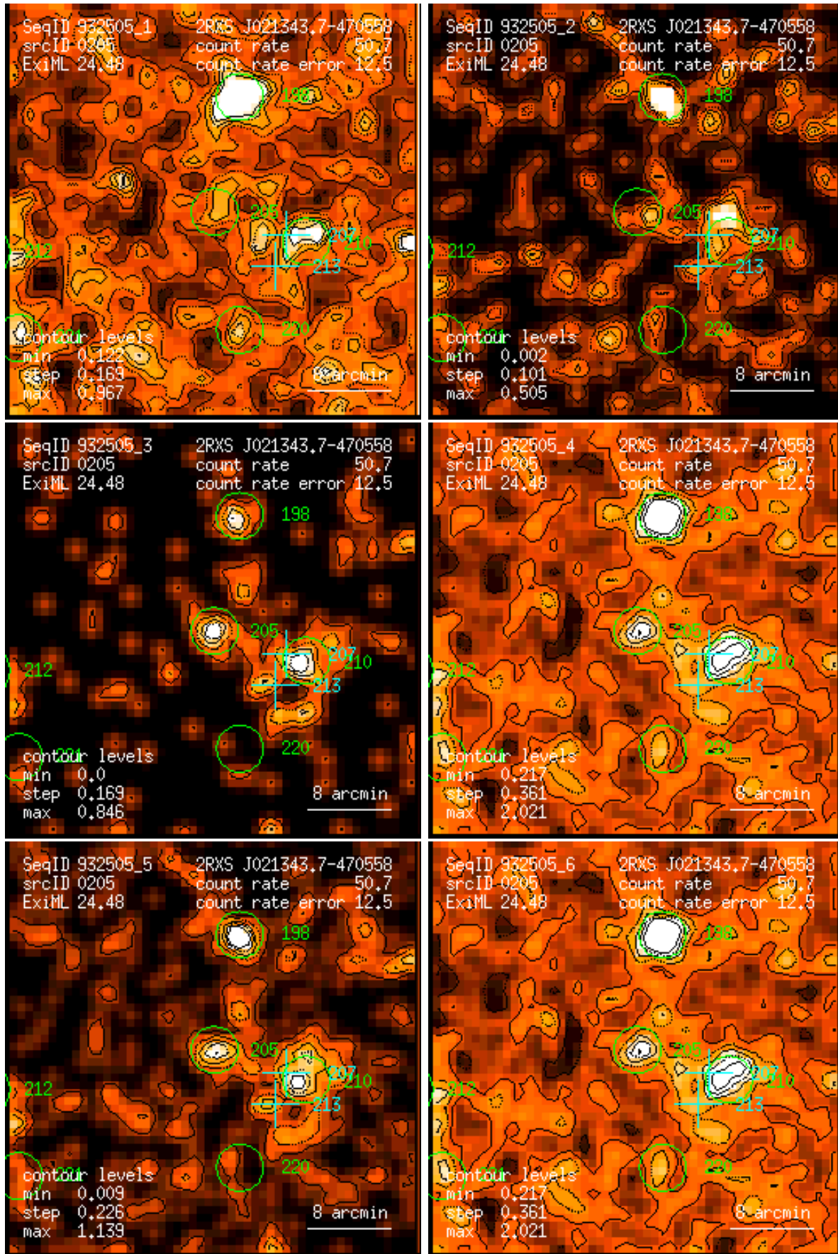
Figure 205: RASS 932505: detection 0205: band rate images, Gaussian filter: (1) PSPC channels 11 – 41, (2) 52 – 90, (3) 91 – 201, (4) 11 – 235, (5) 52 – 201, (6) 11 – 201. Broad band rates in counts/ks. Band rate contour levels in counts/ks/arcmin 2 .
