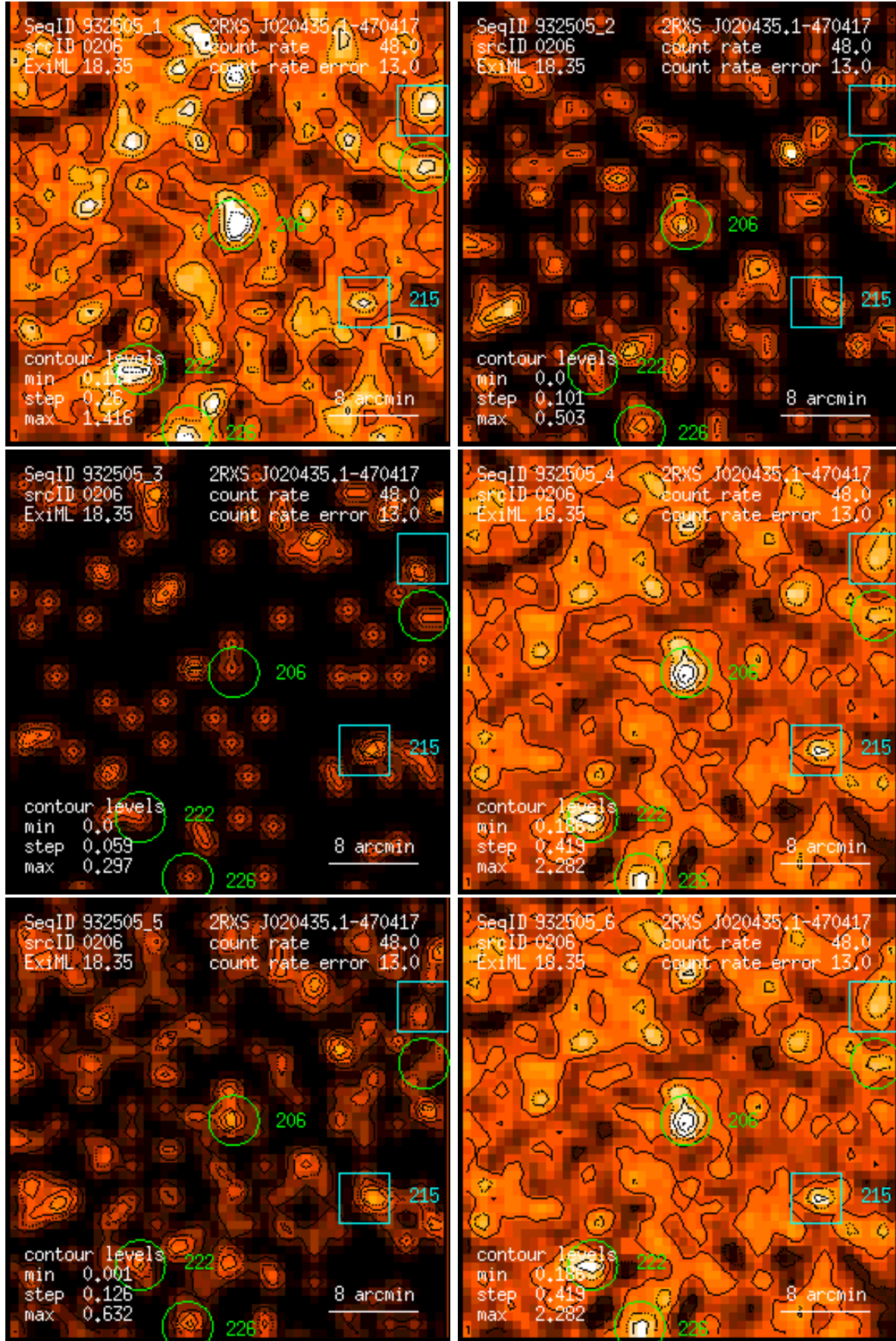
Figure 206: RASS 932505: detection 0206: band rate images, Gaussian filter: (1) PSPC channels 11 – 41, (2) 52 – 90, (3) 91 – 201, (4) 11 – 235, (5) 52 – 201, (6) 11 – 201. Broad band rates in counts/ks. Band rate contour levels in counts/ks/arcmin 2 .
