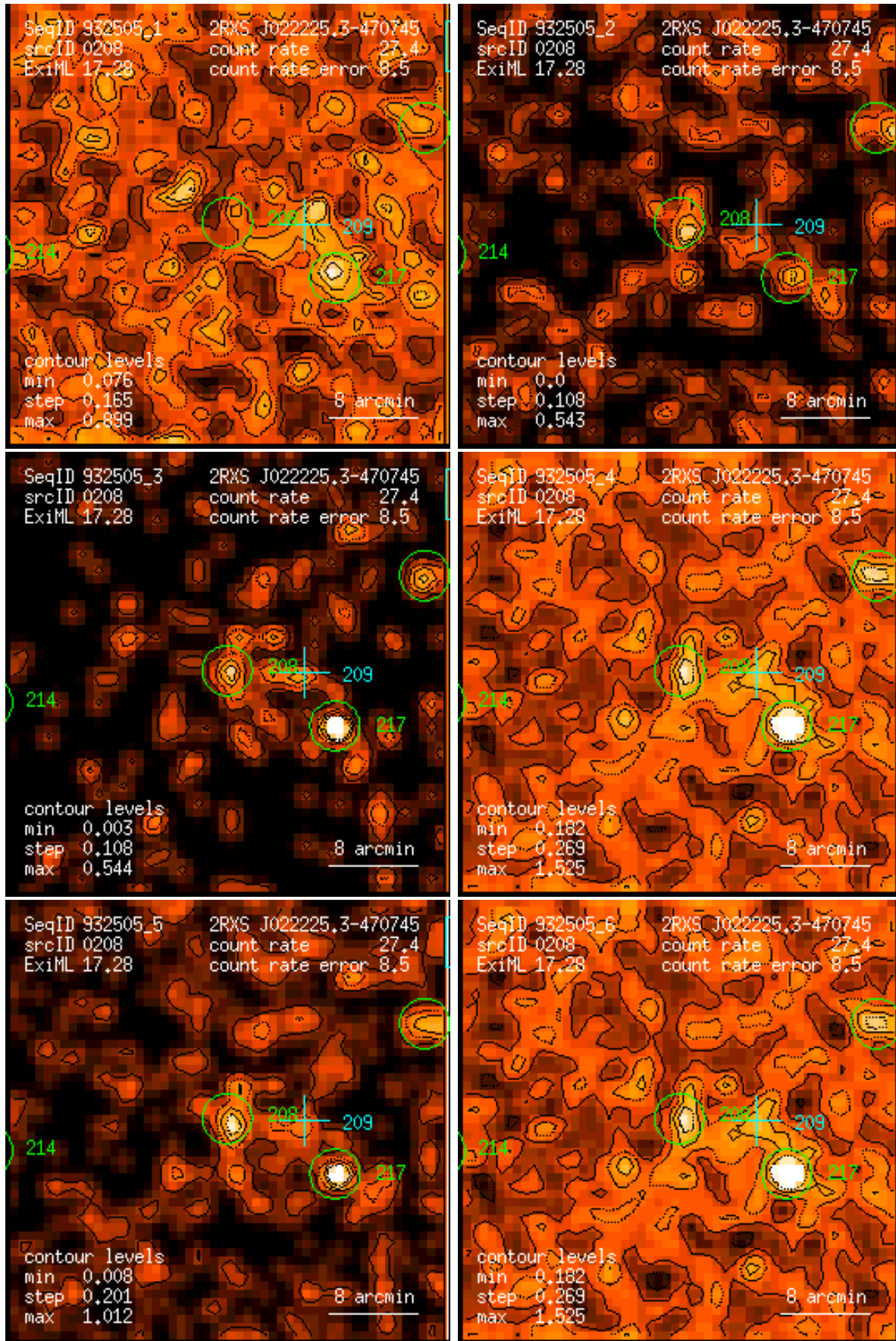
Figure 208: RASS 932505: detection 0208: band rate images, Gaussian filter: (1) PSPC channels 11 – 41, (2) 52 – 90, (3) 91 – 201, (4) 11 – 235, (5) 52 – 201, (6) 11 – 201. Broad band rates in counts/ks. Band rate contour levels in counts/ks/arcmin 2 .
