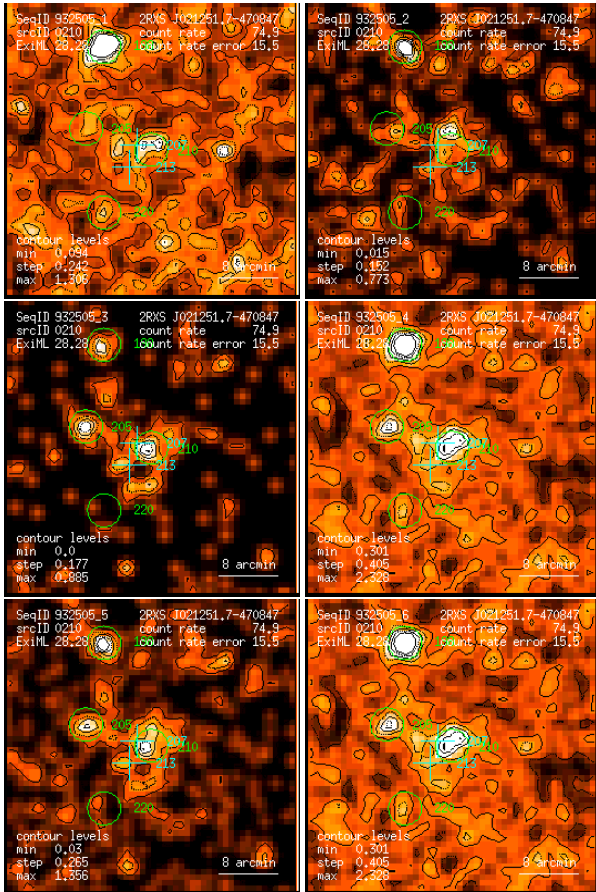
Figure 210: RASS 932505: detection 0210: band rate images, Gaussian filter: (1) PSPC channels 11 – 41, (2) 52 – 90, (3) 91 – 201, (4) 11 – 235, (5) 52 – 201, (6) 11 – 201. Broad band rates in counts/ks. Band rate contour levels in counts/ks/arcmin 2 .
