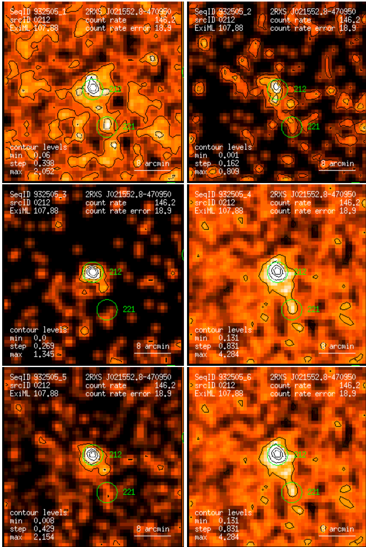
Figure 212: RASS 932505: detection 0212: band rate images, Gaussian filter: (1) PSPC channels 11 – 41, (2) 52 – 90, (3) 91 – 201, (4) 11 – 235, (5) 52 – 201, (6) 11 – 201. Broad band rates in counts/ks. Band rate contour levels in counts/ks/arcmin 2 .
